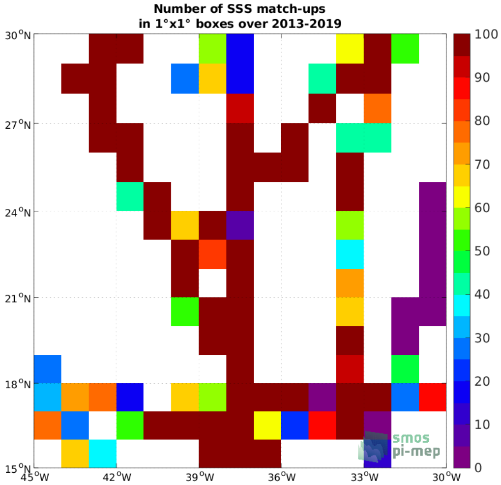
Figure 4: Number of SSS match-ups between TSG (GOSUD-Sailing-ship) SSS and the CCI SSS L4 Merged-OI v3.2 - 7-day running (ESA) SSS product for the SPURS 1 Pi-MEP region over 1^\circ \times 1^\circ boxes and for the full satellite product period.
