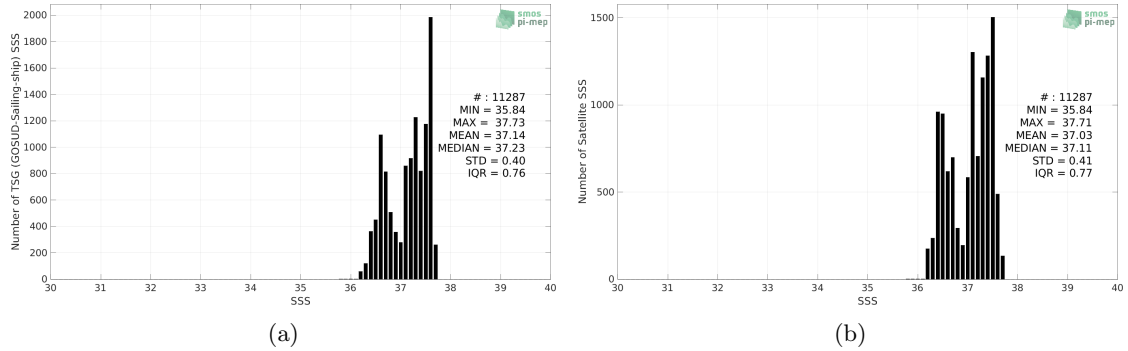
Figure 2: Histograms of SSS from TSG (GOSUD-Sailing-ship) (a) and CCI SSS L4 Merged-OI v3.2 - 7-day running (ESA) (b) considering all match-up pairs per bins of 0.1 over the SPURS 1 Pi-MEP region and for the full satellite product period.
