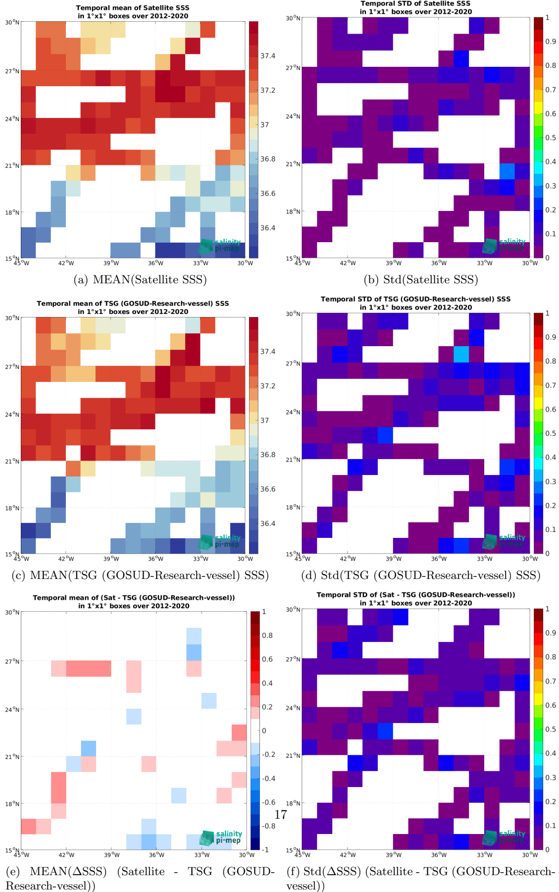
Figure 6: Temporal mean (left) and Std (right) of SSS from CCI SSS L4 Merged-OI v3.2 - 7-day running (ESA) (top), TSG (GOSUD-Research-vessel) (middle), and of \Delta SSS (Satellite - TSG (GOSUD-Research-vessel)). Only match-up pairs are used to generate these maps.
