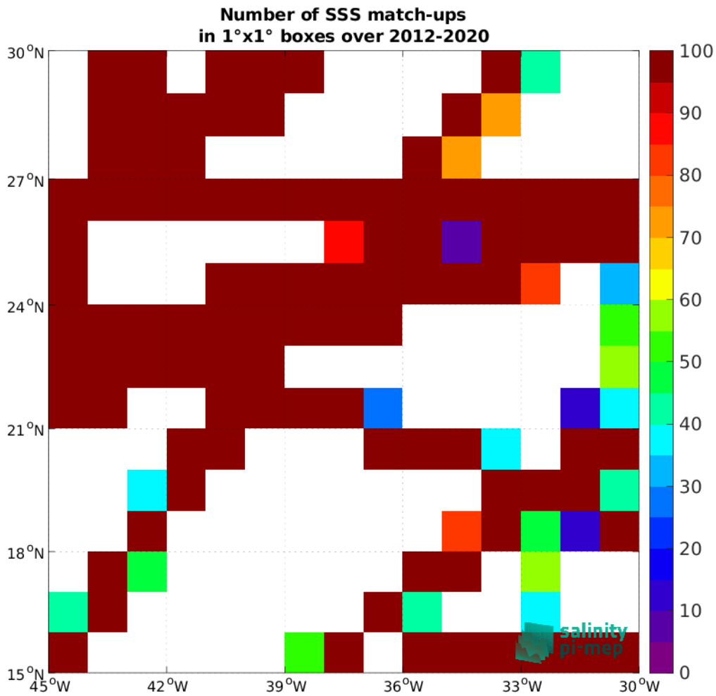
Figure 4: Number of SSS match-ups between TSG (GOSUD-Research-vessel) SSS and the CCI SSS L4 Merged-OI v3.2 - 7-day running (ESA) SSS product for the SPURS 1 Pi-MEP region over 1°x1° boxes and for the full satellite product period.
