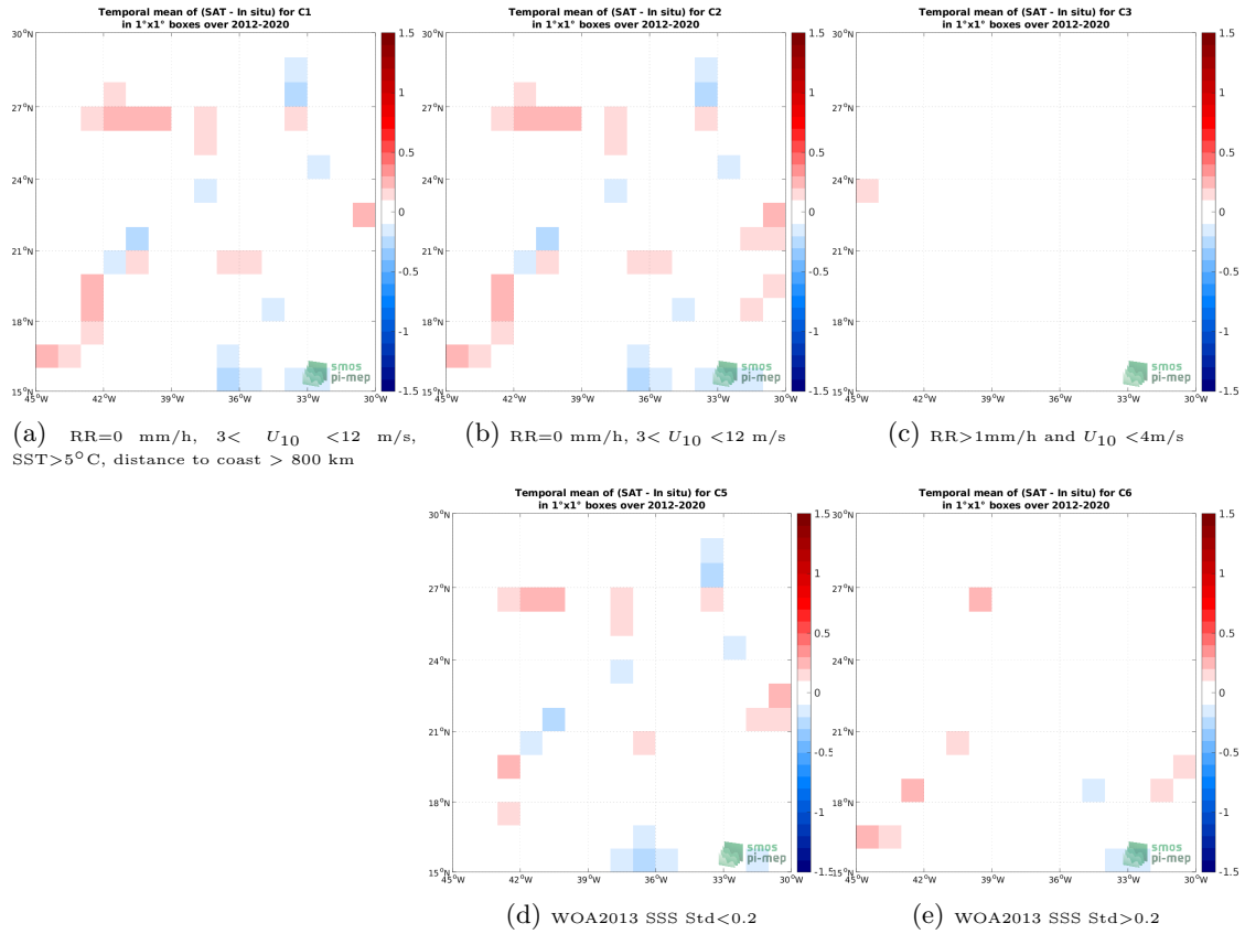
Figure 12: Temporal mean gridded over spatial boxes of size 1^\circ \times 1^\circ of \Delta SSS (CCI SSS L4 Merged-OI v3.2 - 7-day running (ESA) - TSG (GOSUD-Research-vessel)) for 5 different subdatasets corresponding to:RR=0 mm/h, 3 < U_{10} < 12 m/s, SST>5°C, distance to coast > 800 km (a), RR=0 mm/h, 3 < U_{10} < 12 m/s (b), RR>1mm/h and U_{10} < 4 m/s (c), WOA2013 SSS Std<0.2 (d), WOA2013 SSS Std>0.2 (e).
