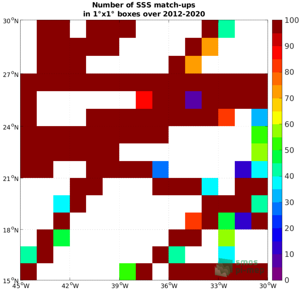
Figure 4: Number of SSS match-ups between TSG (GOSUD-Research-vessel) SSS and the CCI SSS L4 Merged-OI v3.2 - 7-day running (ESA) SSS product for the SPURS 1 Pi-MEP region over 1^\circ \times 1^\circ boxes and for the full satellite product period.
