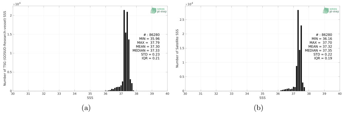
Figure 2: Histograms of SSS from TSG (GOSUD-Research-vessel) (a) and CCI SSS L4 Merged-OI v3.2 - 7-day running (ESA) (b) considering all match-up pairs per bins of 0.1 over the SPURS 1 Pi-MEP region and for the full satellite product period.
