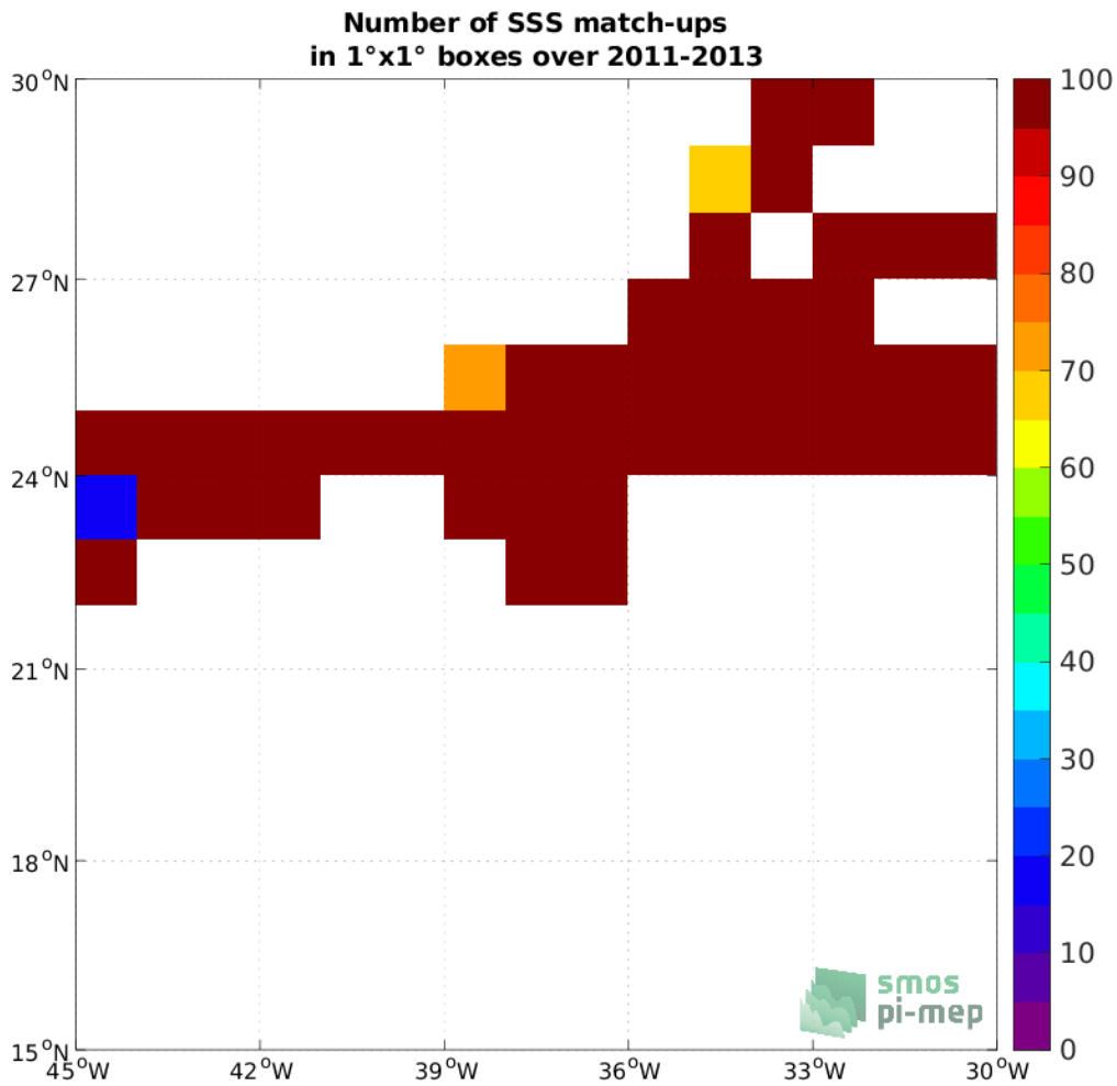
Figure 4: Number of SSS match-ups between TSG (CSIC-UTM) SSS and the CCI SSS L4 Merged-OI v3.2 - 7-day running (ESA) SSS product for the SPURS 1 Pi-MEP region over 1°x1° boxes and for the full satellite product period.
