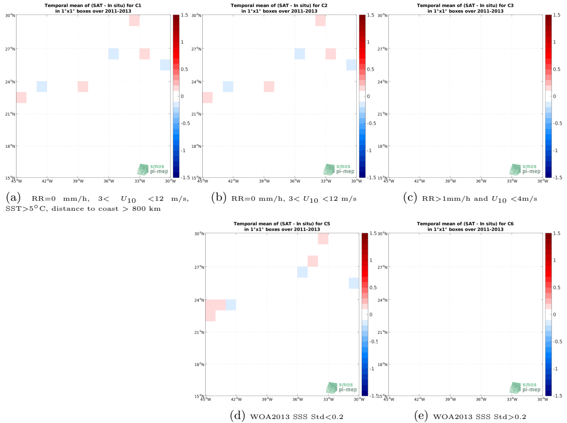
Figure 12: Temporal mean gridded over spatial boxes of size 1^{\circ}\times 1^{\circ} of \Delta\text{SSS} (CCI SSS L4 Merged-OI v3.2 - 7-day running (ESA) - TSG (CSIC-UTM)) for 5 different subdatasets corresponding to:RR=0 mm/h, 3 < U_{10} < 12 m/s, SST >5^{\circ}\text{C} , distance to coast > 800 km (a), RR=0 mm/h, 3 < U_{10} < 12 m/s (b), RR >1 mm/h and U_{10} < 4 m/s (c), WOA2013 SSS Std <0.2 (d), WOA2013 SSS Std >0.2 (e).
