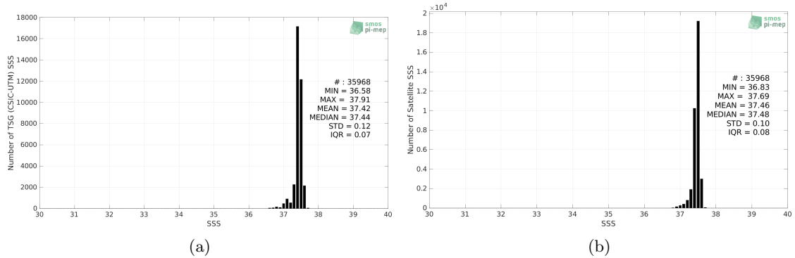
Figure 2: Histograms of SSS from TSG (CSIC-UTM) (a) and CCI SSS L4 Merged-OI v3.2 - 7-day running (ESA) (b) considering all match-up pairs per bins of 0.1 over the SPURS 1 Pi-MEP region and for the full satellite product period.
