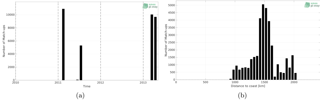
Figure 1: Number of match-ups between TSG (CSIC-UTM) and CCI SSS L4 Merged-OI v3.2 - 7-day running (ESA) SSS as a function of time (a) and as function of the distance to coast (b) over the SPURS 1 Pi-MEP region and for the full satellite product period.
