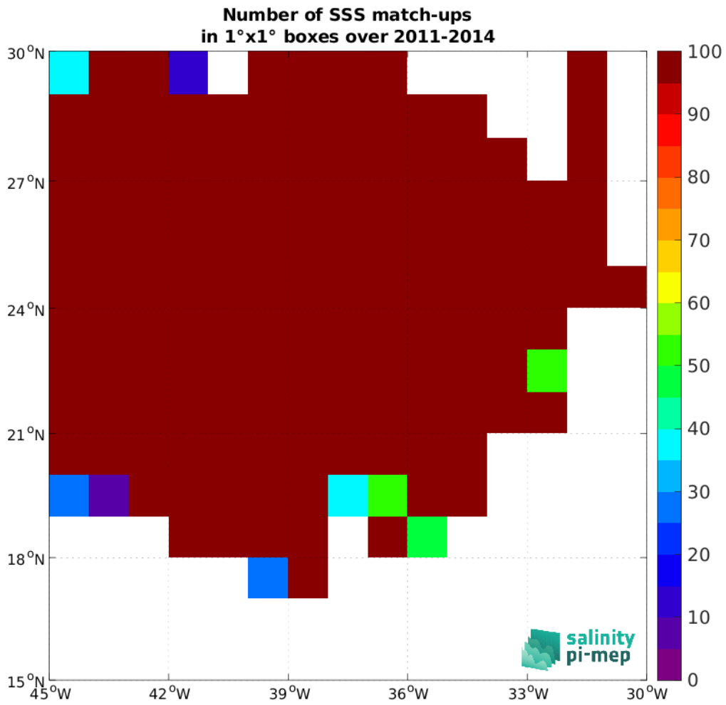
Figure 3: Number of SSS match-ups between Surface drifters SSS and the CCI SSS L4 Merged-OI v3.2 - 7-day running (ESA) SSS product for the SPURS 1 Pi-MEP region over 1°x1° boxes and for the full satellite product period.
