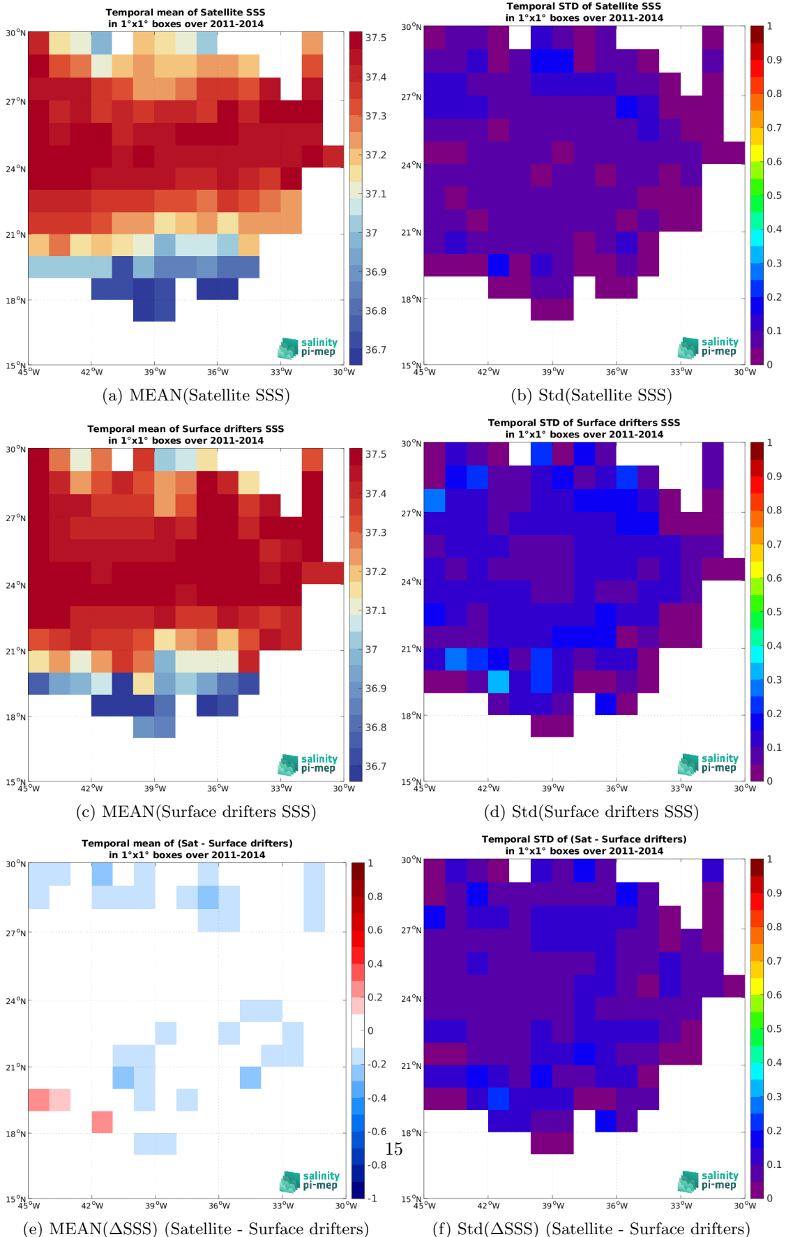
Figure 5: Temporal mean (left) and Std (right) of SSS from CCI SSS L4 Merged-OI v3.2 - 7-day running (ESA) (top), Surface drifters (middle), and of \Delta SSS (Satellite - Surface drifters). Only match-up pairs are used to generate these maps.
