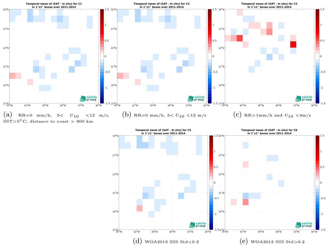
Figure 11: Temporal mean gridded over spatial boxes of size 1^\circ \times 1^\circ of \Delta SSS (CCI SSS L4 Merged-OI v3.2 - 7-day running (ESA) - Surface drifters) for 5 different subdatasets corresponding to:RR=0 mm/h, 3 < U_{10} < 12 m/s, SST >5^\circ C, distance to coast > 800 km (a), RR=0 mm/h, 3 < U_{10} < 12 m/s (b), RR >1 mm/h and U_{10} < 4 m/s (c), WOA2013 SSS Std <0.2 (d), WOA2013 SSS Std >0.2 (e).
