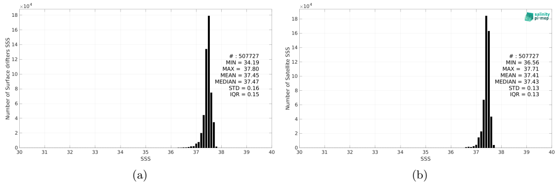
Figure 2: Histograms of SSS from Surface drifters (a) and CCI SSS L4 Merged-OI v3.2 - 7-day running (ESA) (b) considering all match-up pairs per bins of 0.1 over the SPURS 1 Pi-MEP region and for the full satellite product period.
