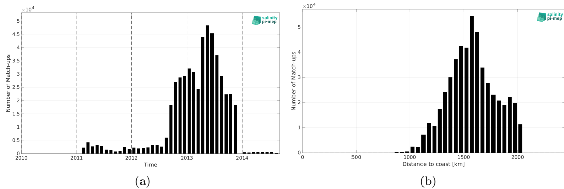
Figure 1: Number of match-ups between Surface drifters and CCI SSS L4 Merged-OI v3.2 - 7-day running (ESA) SSS as a function of time (a) and as function of the distance to coast (b) over the SPURS 1 Pi-MEP region and for the full satellite product period.
