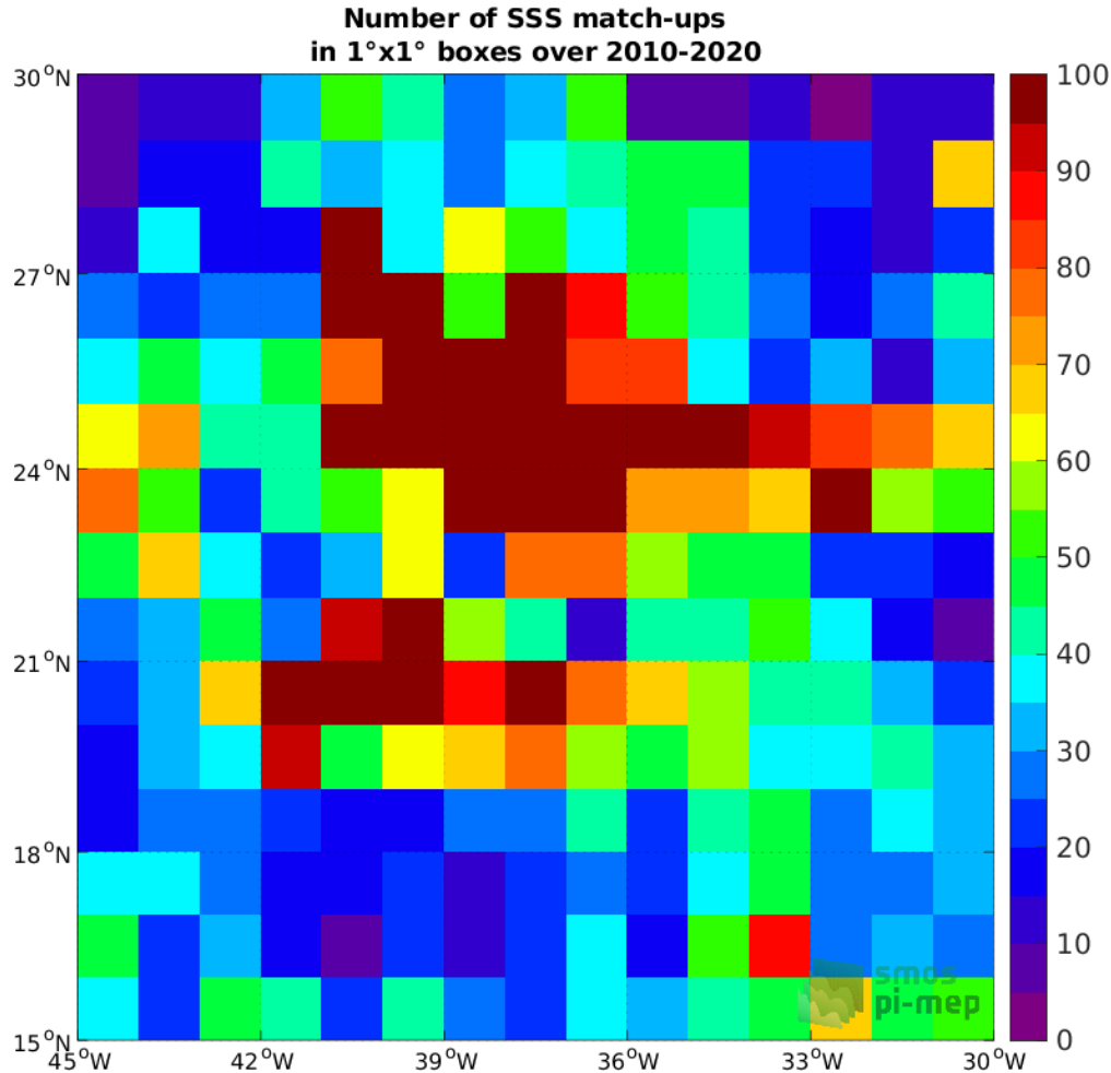
Figure 4: Number of SSS match-ups between Argo SSS and the CCI SSS L4 Merged-OI v3.2 - 7-day running (ESA) SSS product for the SPURS 1 Pi-MEP region over 1^\circ \times 1^\circ boxes and for the full satellite product period.
