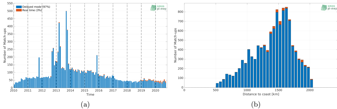
Figure 1: Number of match-ups between Argo and CCI SSS L4 Merged-OI v3.2 - 7-day running (ESA) SSS as a function of time (a) and as function of the distance to coast (b) over the SPURS 1 Pi-MEP region and for the full satellite product period.
