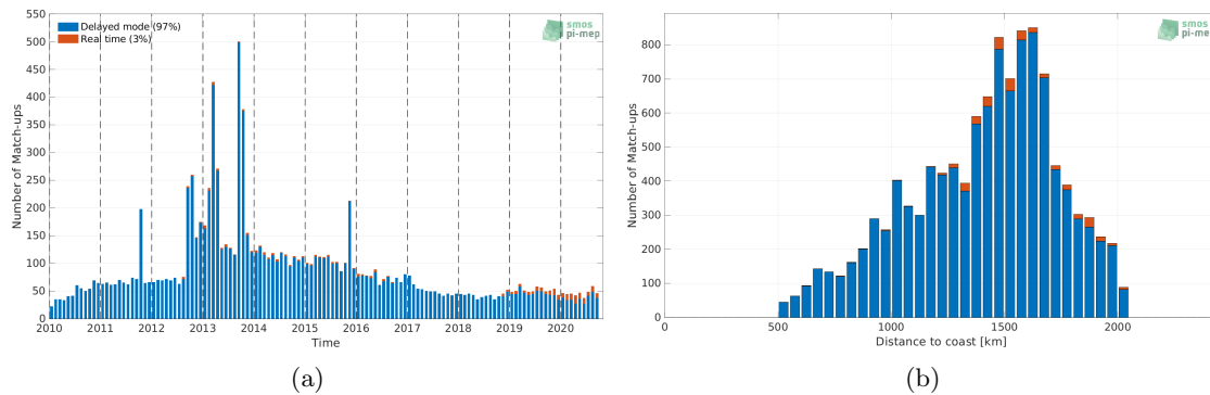
Figure 1: Number of match-ups between Argo and CCI SSS L4 Merged-OI v3.2 - 7-day running (ESA) SSS as a function of time (a) and as function of the distance to coast (b) over the SPURS 1 Pi-MEP region and for the full satellite product period.
