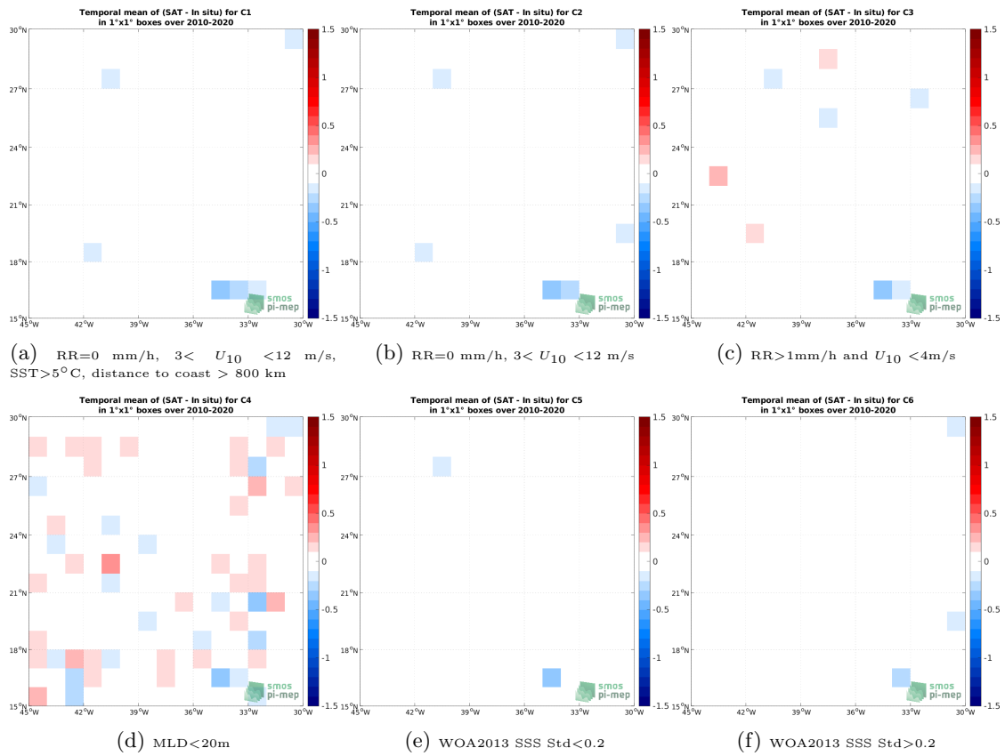
Figure 12: Temporal mean gridded over spatial boxes of size 1^\circ \times 1^\circ of \Delta SSS (CCI SSS L4 Merged-OI v3.2 - 7-day running (ESA) - Argo) for 6 different subdatasets corresponding to:RR=0 mm/h, 3 < U_{10} < 12 m/s, SST >5^\circ\text{C} , distance to coast > 800 km (a), RR=0 mm/h, 3 < U_{10} < 12 m/s (b), RR >1 mm/h and U_{10} < 4 m/s (c),MLD <20 m (d),WOA2013 SSS Std <0.2 (e),WOA2013 SSS Std >0.2 (f).
