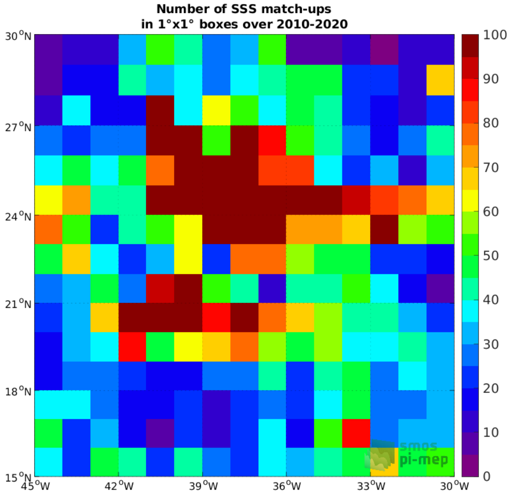
Figure 4: Number of SSS match-ups between Argo SSS and the CCI SSS L4 Merged-OI v3.2 - 7-day running (ESA) SSS product for the SPURS 1 Pi-MEP region over 1°x1° boxes and for the full satellite product period.
