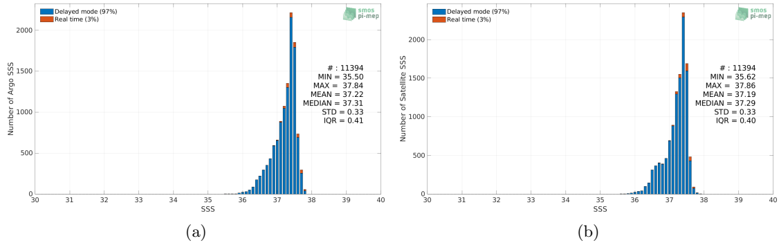
Figure 2: Histograms of SSS from Argo (a) and CCI SSS L4 Merged-OI v3.2 - 7-day running (ESA) (b) considering all match-up pairs per bins of 0.1 over the SPURS 1 Pi-MEP region and for the full satellite product period.
