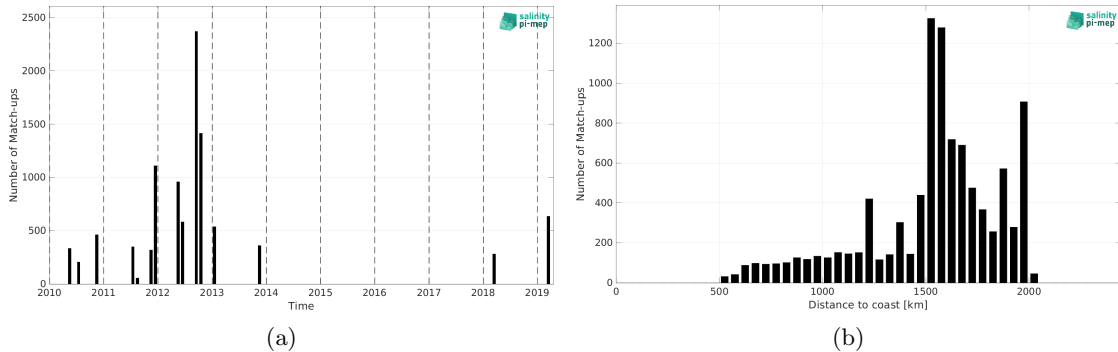
Figure 1: Number of match-ups between TSG (SAMOS) and CCI SSS L4 Merged-OI v3.2 - 30-day running (ESA) SSS as a function of time (a) and as function of the distance to coast (b) over the SPURS 1 Pi-MEP region and for the full satellite product period.
