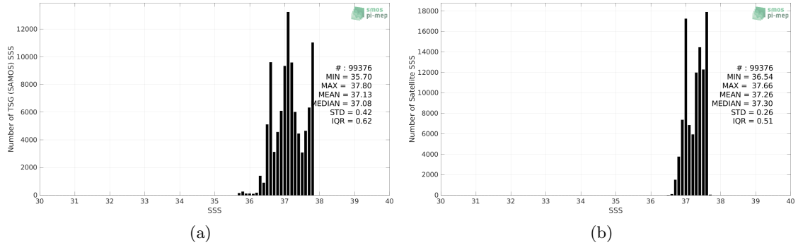
Figure 2: Histograms of SSS from TSG (SAMOS) (a) and CCI SSS L4 Merged-OI v3.2 - 30-day running (ESA) (b) considering all match-up pairs per bins of 0.1 over the SPURS 1 Pi-MEP region and for the full satellite product period.
