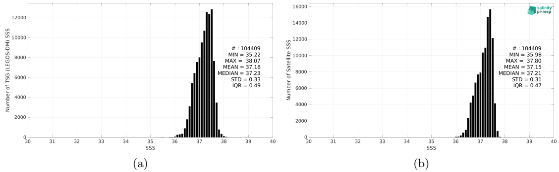
Figure 2: Histograms of SSS from TSG (LEGOS-DM) (a) and CCI SSS L4 Merged-OI v3.2 - 30-day running (ESA) (b) considering all match-up pairs per bins of 0.1 over the SPURS 1 Pi-MEP region and for the full satellite product period.
