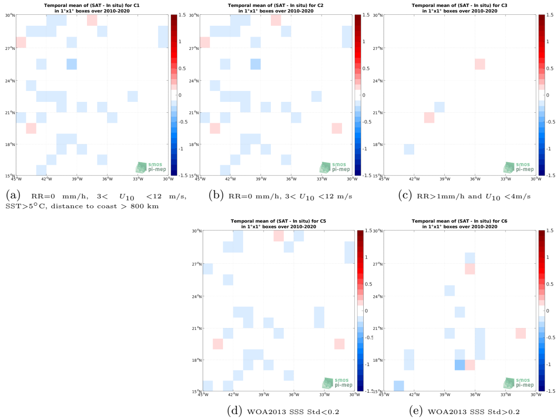
Figure 12: Temporal mean gridded over spatial boxes of size 1^{\circ}\times 1^{\circ} of \Delta\text{SSS} (CCI SSS L4 Merged-OI v3.2 - 30-day running (ESA) - TSG (LEGOS-DM)) for 5 different subdatasets corresponding to:RR=0 mm/h, 3 < U_{10} < 12 m/s, SST >5^{\circ}\text{C} , distance to coast > 800 km (a), RR=0 mm/h, 3 < U_{10} < 12 m/s (b), RR >1 mm/h and U_{10} < 4 m/s (c), WOA2013 SSS Std <0.2 (d), WOA2013 SSS Std >0.2 (e).
