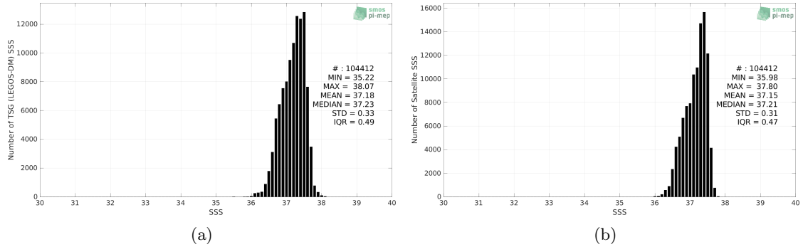
Figure 2: Histograms of SSS from TSG (LEGOS-DM) (a) and CCI SSS L4 Merged-OI v3.2 - 30-day running (ESA) (b) considering all match-up pairs per bins of 0.1 over the SPURS 1 Pi-MEP region and for the full satellite product period.
