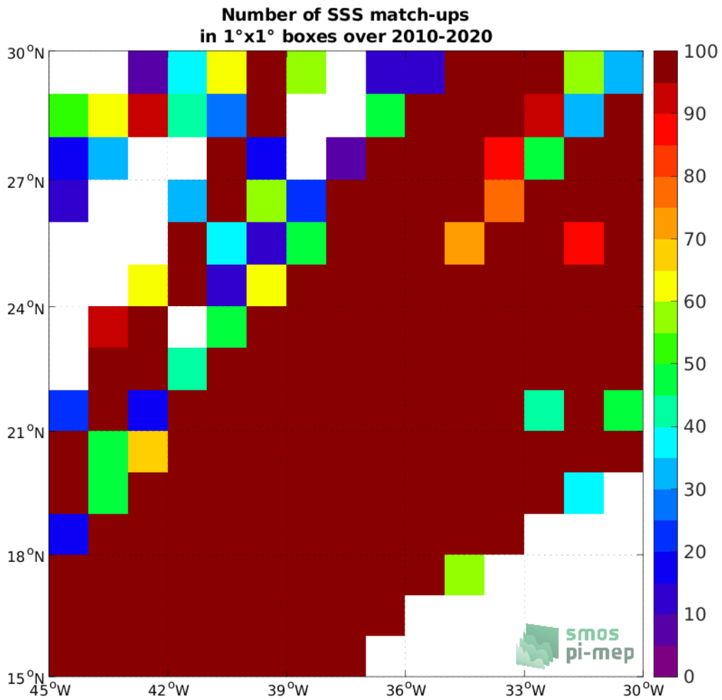
Figure 4: Number of SSS match-ups between TSG (LEGOS-DM) SSS and the CCI SSS L4 Merged-OI v3.2 - 30-day running (ESA) SSS product for the SPURS 1 Pi-MEP region over 1^\circ \times 1^\circ boxes and for the full satellite product period.
