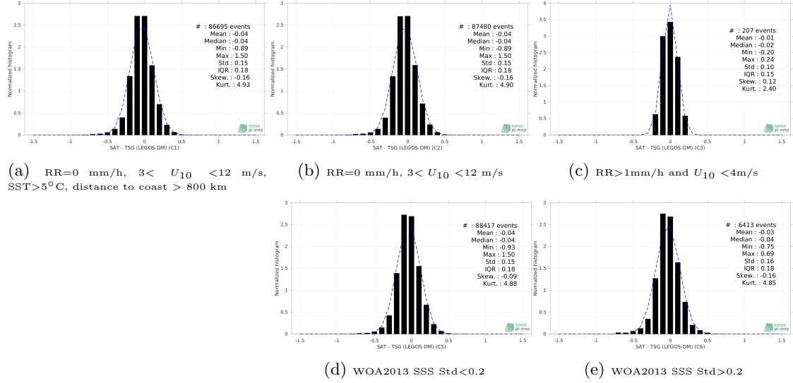
Figure 13: Normalized histogram of \Delta SSS (CCI SSS L4 Merged-OI v3.2 - 30-day running (ESA) - TSG (LEGOS-DM)) for 5 different subdatasets corresponding to: RR=0 mm/h, 3 < U_{10} < 12 m/s, SST > 5°C, distance to coast > 800 km (a), RR=0 mm/h, 3 < U_{10} < 12 m/s (b), RR > 1mm/h and U_{10} < 4 m/s (c), WOA2013 SSS Std < 0.2 (d), WOA2013 SSS Std > 0.2 (e).
