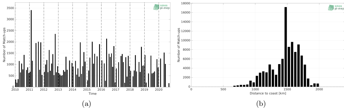
Figure 1: Number of match-ups between TSG (LEGOS-DM) and CCI SSS L4 Merged-OI v3.2 - 30-day running (ESA) SSS as a function of time (a) and as function of the distance to coast (b) over the SPURS 1 Pi-MEP region and for the full satellite product period.
