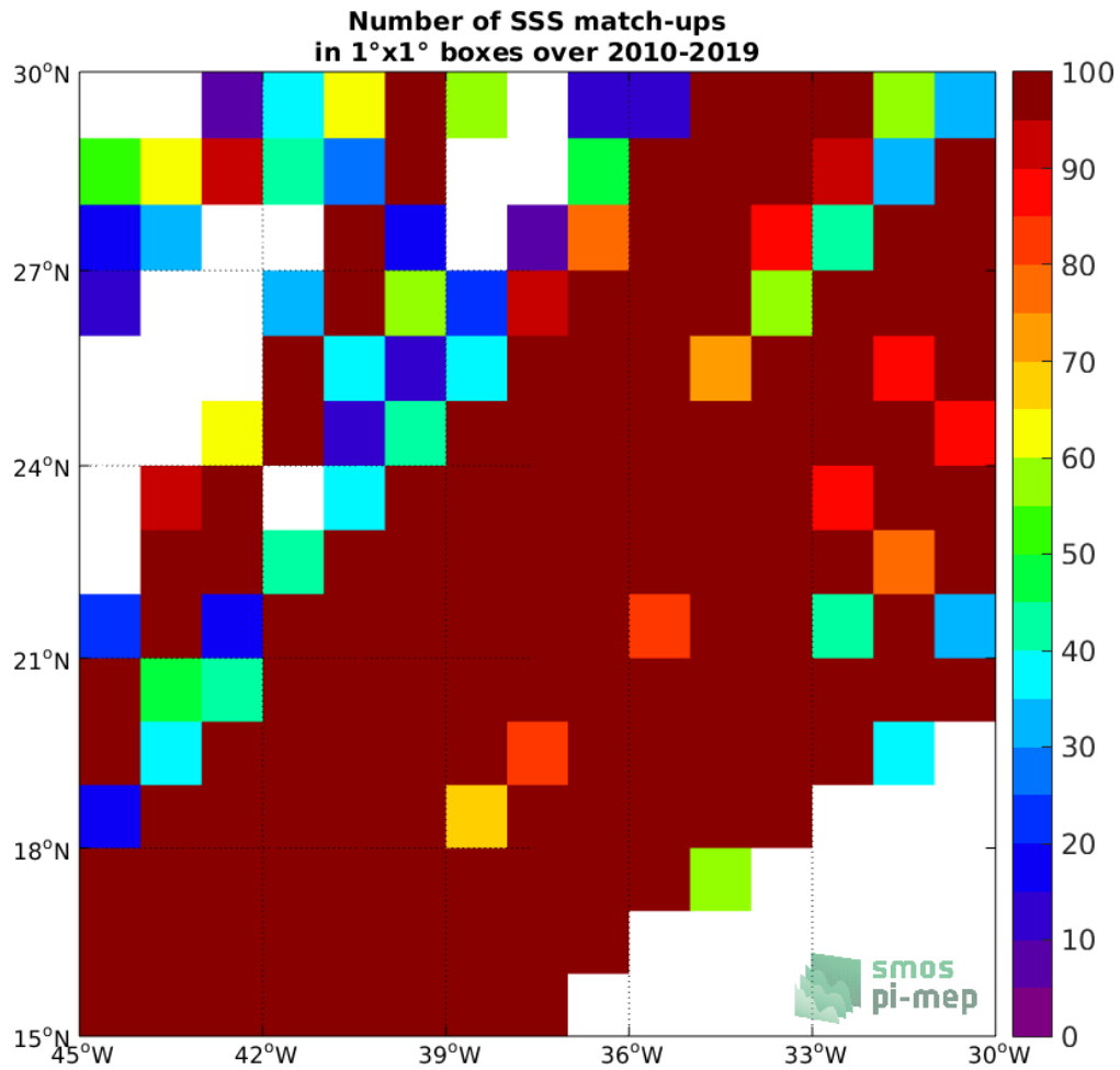
Figure 4: Number of SSS match-ups between TSG (LEGOS-DM) SSS and the CCI SSS L4 Merged-OI v3.2 - 30-day running (ESA) SSS product for the SPURS 1 Pi-MEP region over 1°x1° boxes and for the full satellite product period.
