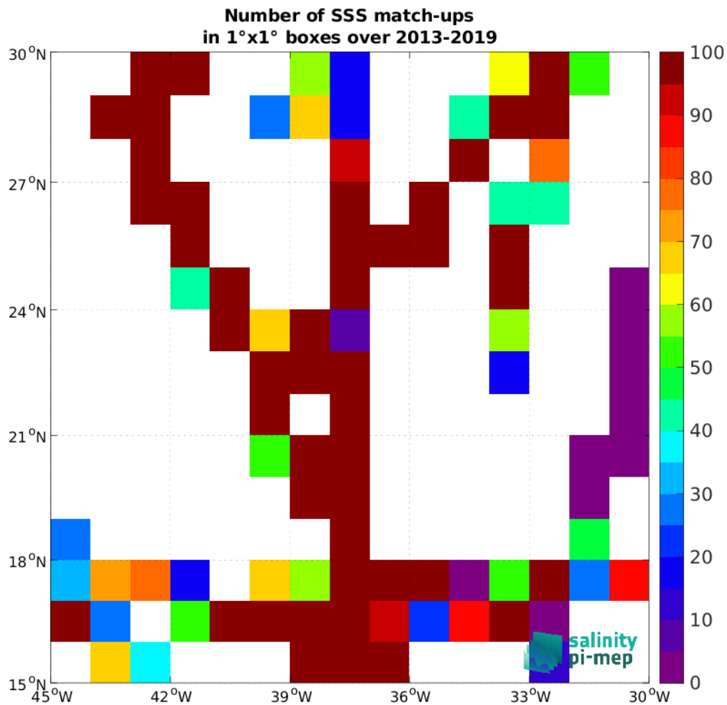
Figure 4: Number of SSS match-ups between TSG (GOSUD-Sailing-ship) SSS and the CCI SSS L4 Merged-OI v3.2 - 30-day running (ESA) SSS product for the SPURS 1 Pi-MEP region over 1^\circ \times 1^\circ boxes and for the full satellite product period.
