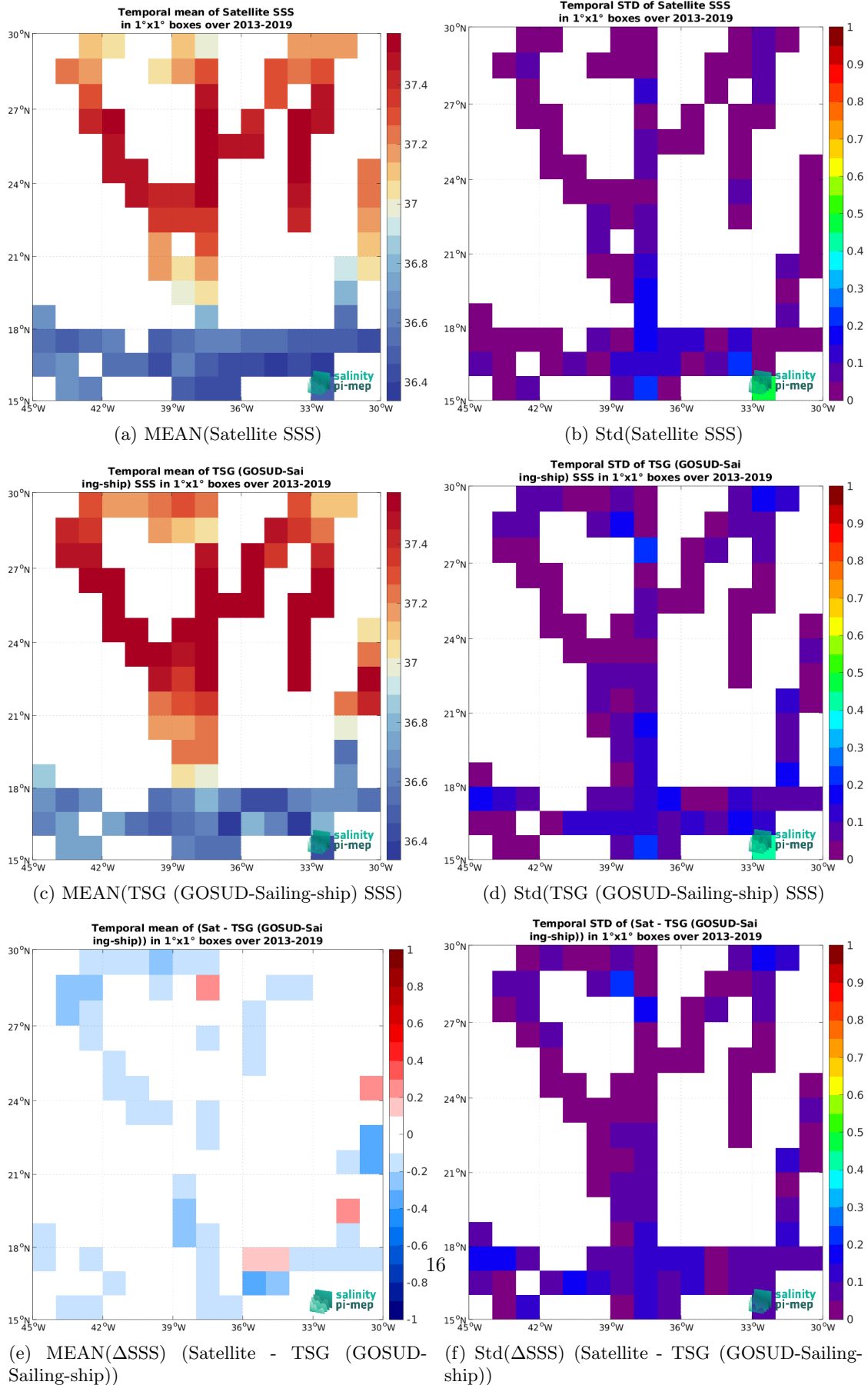
Figure 6: Temporal mean (left) and Std (right) of SSS from CCI SSS L4 Merged-OI v3.2 - 30-day running (ESA) (top), TSG (GOSUD-Sailing-ship) (middle), and of \Delta SSS (Satellite - TSG (GOSUD-Sailing-ship)). Only match-up pairs are used to generate these maps.
