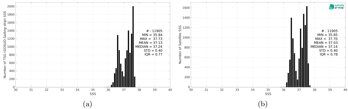
Figure 2: Histograms of SSS from TSG (GOSUD-Sailing-ship) (a) and CCI SSS L4 Merged-OI v3.2 - 30-day running (ESA) (b) considering all match-up pairs per bins of 0.1 over the SPURS 1 Pi-MEP region and for the full satellite product period.
