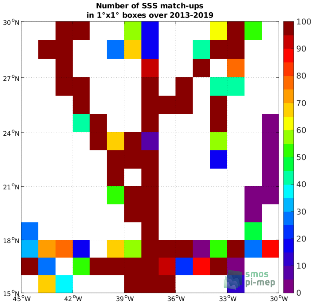
Figure 4: Number of SSS match-ups between TSG (GOSUD-Sailing-ship) SSS and the CCI SSS L4 Merged-OI v3.2 - 30-day running (ESA) SSS product for the SPURS 1 Pi-MEP region over 1°×1° boxes and for the full satellite product period.
