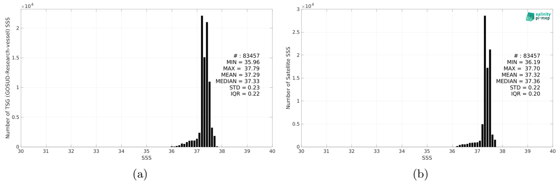
Figure 2: Histograms of SSS from TSG (GOSUD-Research-vessel) (a) and CCI SSS L4 Merged-OI v3.2 - 30-day running (ESA) (b) considering all match-up pairs per bins of 0.1 over the SPURS 1 Pi-MEP region and for the full satellite product period.
