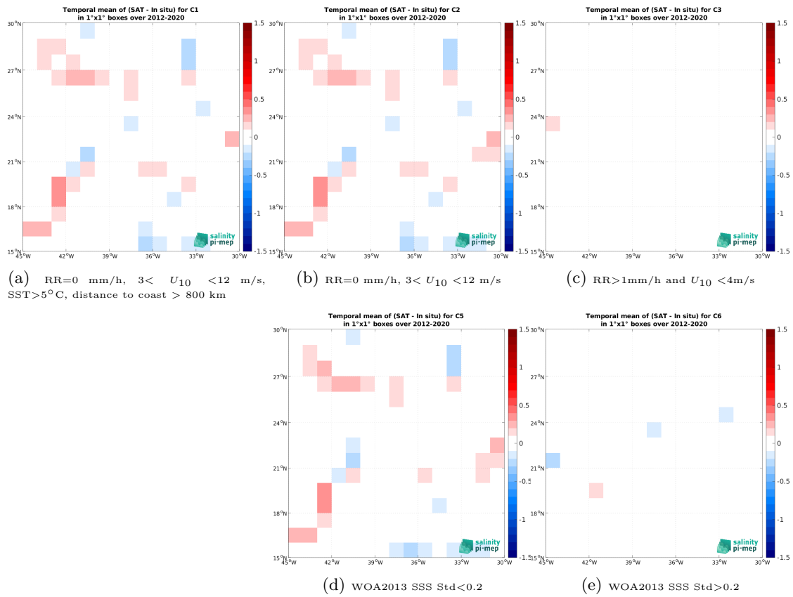
Figure 12: Temporal mean gridded over spatial boxes of size 1^\circ \times 1^\circ of \Delta SSS (CCI SSS L4 Merged-OI v3.2 - 30-day running (ESA) - TSG (GOSUD-Research-vessel)) for 5 different subdatasets corresponding to: RR=0 mm/h, 3 < U_{10} < 12 m/s, SST > 5°C, distance to coast > 800 km (a), RR=0 mm/h, 3 < U_{10} < 12 m/s (b), RR > 1mm/h and U_{10} < 4 m/s (c), WOA2013 SSS Std < 0.2 (d), WOA2013 SSS Std > 0.2 (e).
