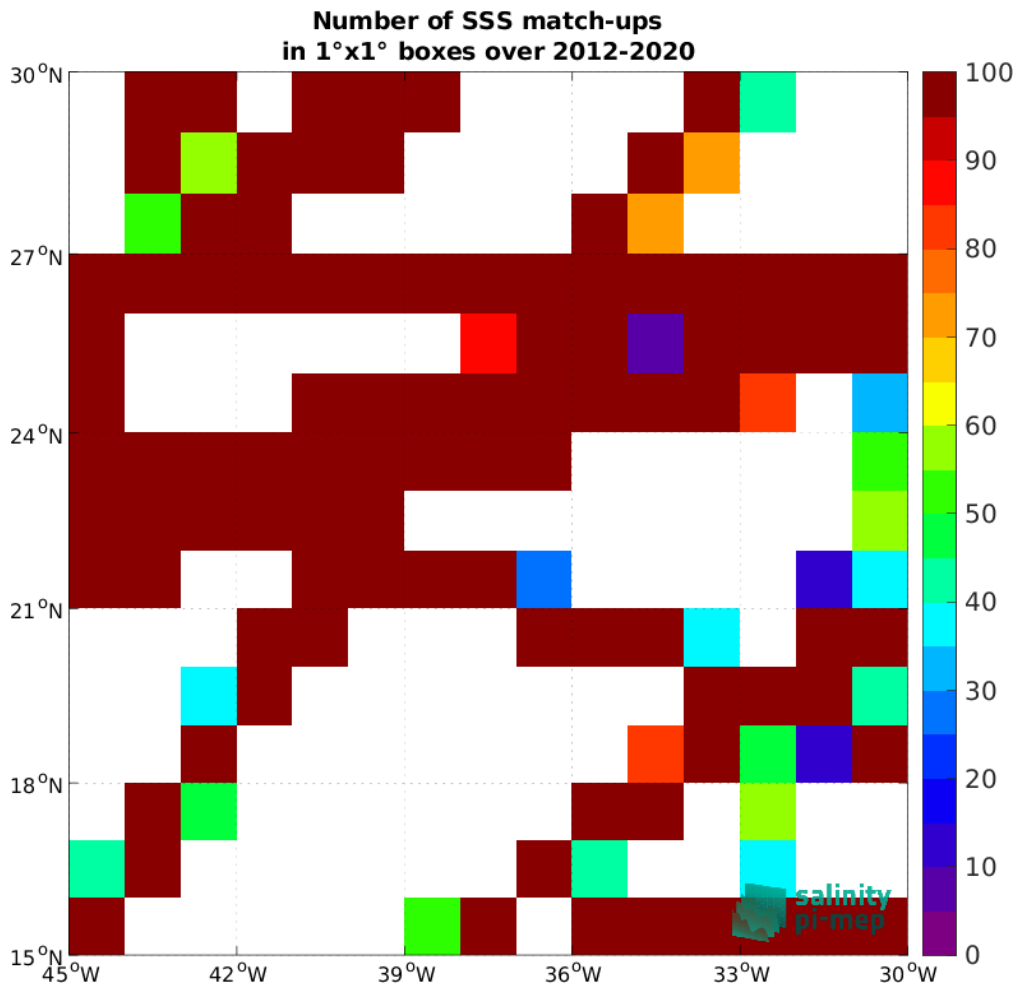
Figure 4: Number of SSS match-ups between TSG (GOSUD-Research-vessel) SSS and the CCI SSS L4 Merged-OI v3.2 - 30-day running (ESA) SSS product for the SPURS 1 Pi-MEP region over 1°x1° boxes and for the full satellite product period.
