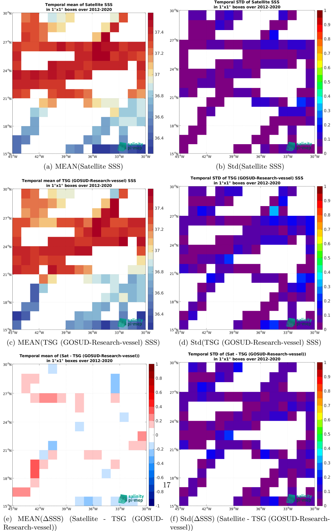
Figure 6: Temporal mean (left) and Std (right) of SSS from CCI SSS L4 Merged-OI v3.2 - 30-day running (ESA) (top), TSG (GOSUD-Research-vessel) (middle), and of \Delta SSS (Satellite - TSG (GOSUD-Research-vessel)). Only match-up pairs are used to generate these maps.
