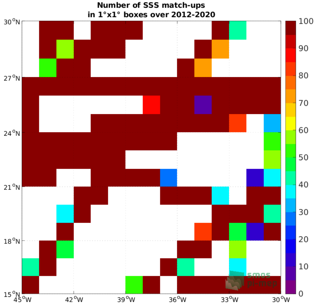
Figure 4: Number of SSS match-ups between TSG (GOSUD-Research-vessel) SSS and the CCI SSS L4 Merged-OI v3.2 - 30-day running (ESA) SSS product for the SPURS 1 Pi-MEP region over 1^\circ \times 1^\circ boxes and for the full satellite product period.
