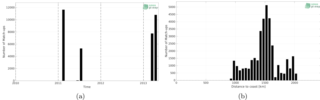
Figure 1: Number of match-ups between TSG (CSIC-UTM) and CCI SSS L4 Merged-OI v3.2 - 30-day running (ESA) SSS as a function of time (a) and as function of the distance to coast (b) over the SPURS 1 Pi-MEP region and for the full satellite product period.
