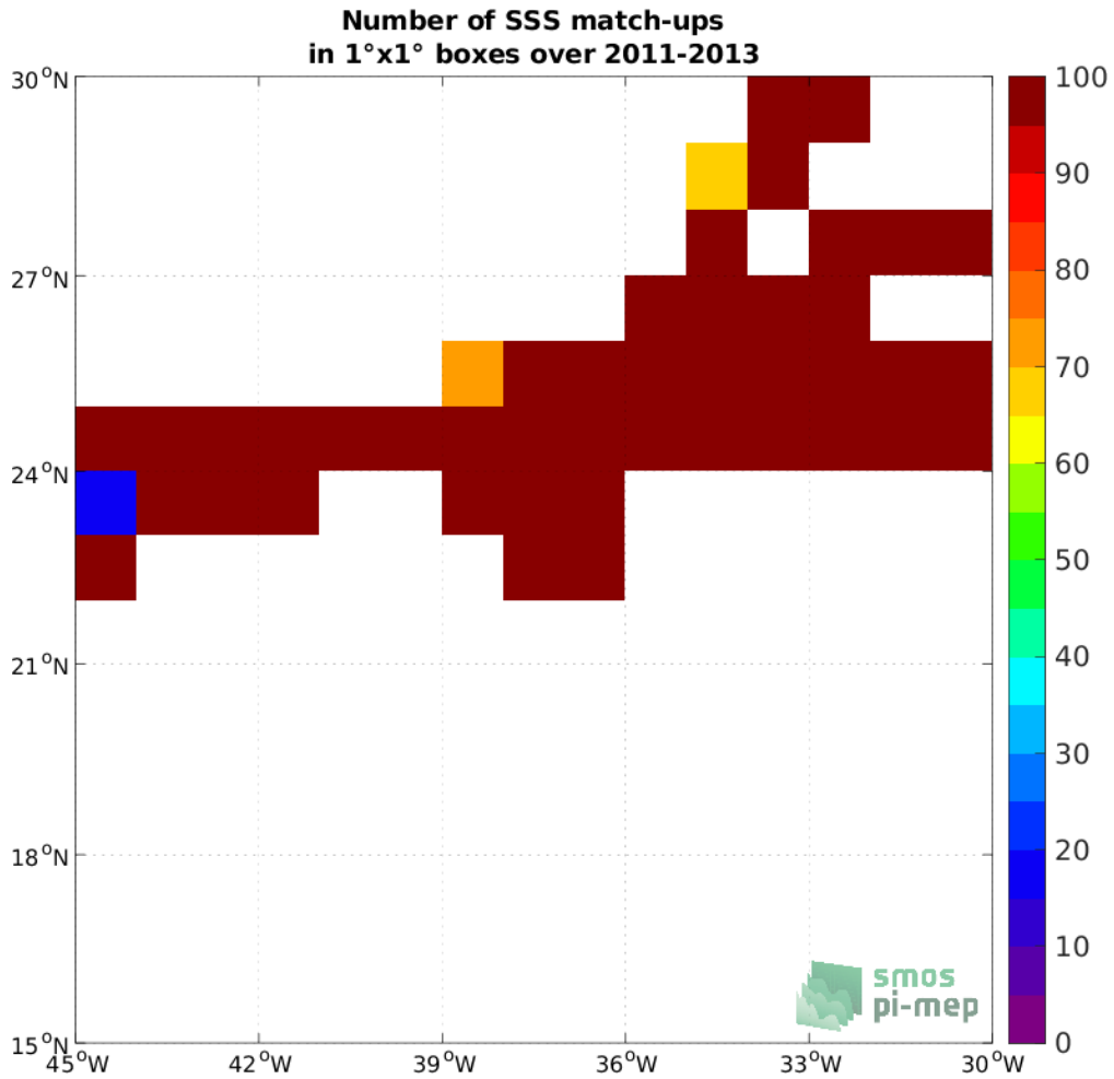
Figure 4: Number of SSS match-ups between TSG (CSIC-UTM) SSS and the CCI SSS L4 Merged-OI v3.2 - 30-day running (ESA) SSS product for the SPURS 1 Pi-MEP region over 1^\circ \times 1^\circ boxes and for the full satellite product period.
