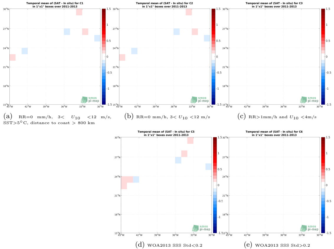
Figure 12: Temporal mean gridded over spatial boxes of size 1^{\circ}\times 1^{\circ} of \Delta\text{SSS} (CCI SSS L4 Merged-OI v3.2 - 30-day running (ESA) - TSG (CSIC-UTM)) for 5 different subdatasets corresponding to:RR=0 mm/h, 3 < U_{10} < 12 m/s, SST >5^{\circ}\text{C} , distance to coast > 800 km (a), RR=0 mm/h, 3 < U_{10} < 12 m/s (b), RR >1 mm/h and U_{10} < 4 m/s (c), WOA2013 SSS Std <0.2 (d), WOA2013 SSS Std >0.2 (e).
