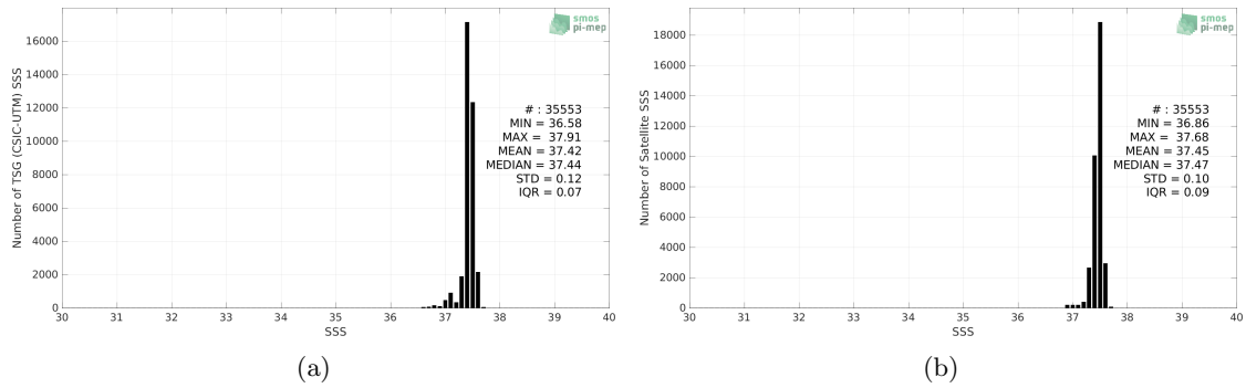
Figure 2: Histograms of SSS from TSG (CSIC-UTM) (a) and CCI SSS L4 Merged-OI v3.2 - 30-day running (ESA) (b) considering all match-up pairs per bins of 0.1 over the SPURS 1 Pi-MEP region and for the full satellite product period.
