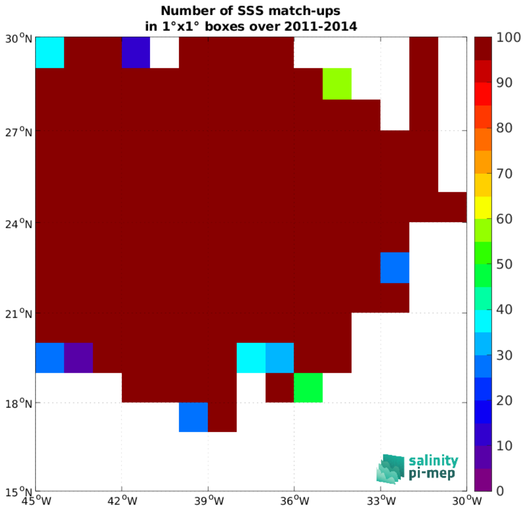
Figure 3: Number of SSS match-ups between Surface drifters SSS and the CCI SSS L4 Merged-OI v3.2 - 30-day running (ESA) SSS product for the SPURS 1 Pi-MEP region over 1^\circ \times 1^\circ boxes and for the full satellite product period.
