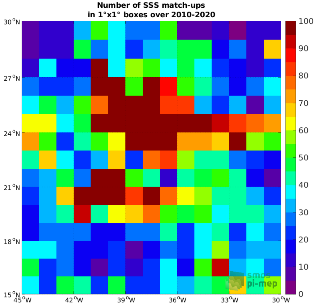
Figure 4: Number of SSS match-ups between Argo SSS and the CCI SSS L4 Merged-OI v3.2 - 30-day running (ESA) SSS product for the SPURS 1 Pi-MEP region over 1^\circ \times 1^\circ boxes and for the full satellite product period.
