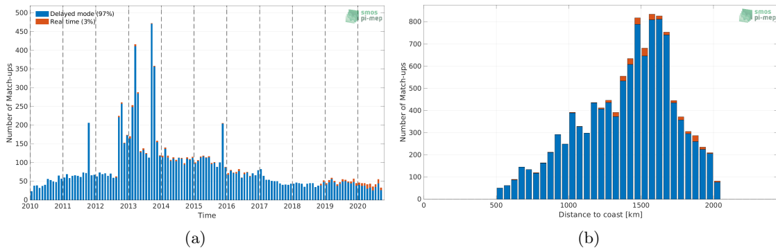
Figure 1: Number of match-ups between Argo and CCI SSS L4 Merged-OI v3.2 - 30-day running (ESA) SSS as a function of time (a) and as function of the distance to coast (b) over the SPURS 1 Pi-MEP region and for the full satellite product period.
