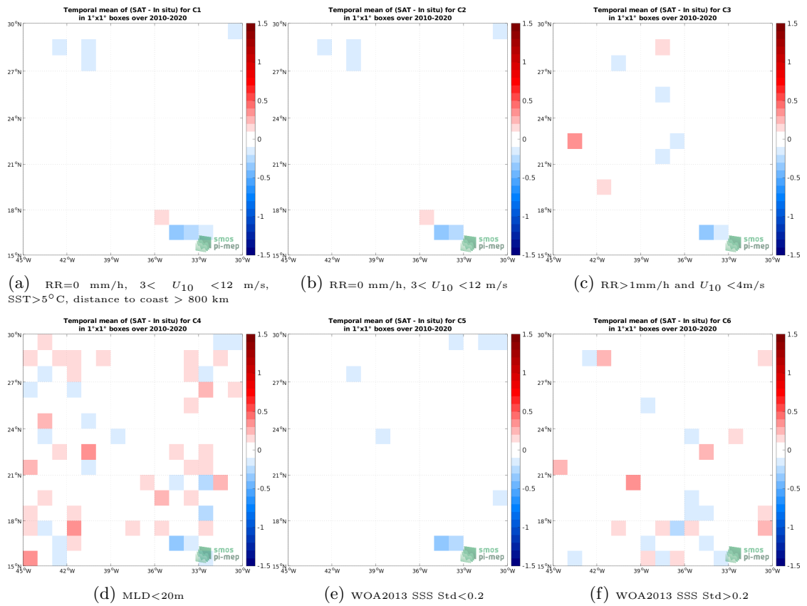
Figure 12: Temporal mean gridded over spatial boxes of size 1^\circ \times 1^\circ of \Delta SSS (CCI SSS L4 Merged-OI v3.2 - 30-day running (ESA) - Argo) for 6 different subdatasets corresponding to:RR=0 mm/h, 3 < U_{10} < 12 m/s, SST >5^\circ C, distance to coast > 800 km (a), RR=0 mm/h, 3 < U_{10} < 12 m/s (b), RR >1 mm/h and U_{10} < 4 m/s (c),MLD <20 m (d),WOA2013 SSS Std <0.2 (e),WOA2013 SSS Std >0.2 (f).
