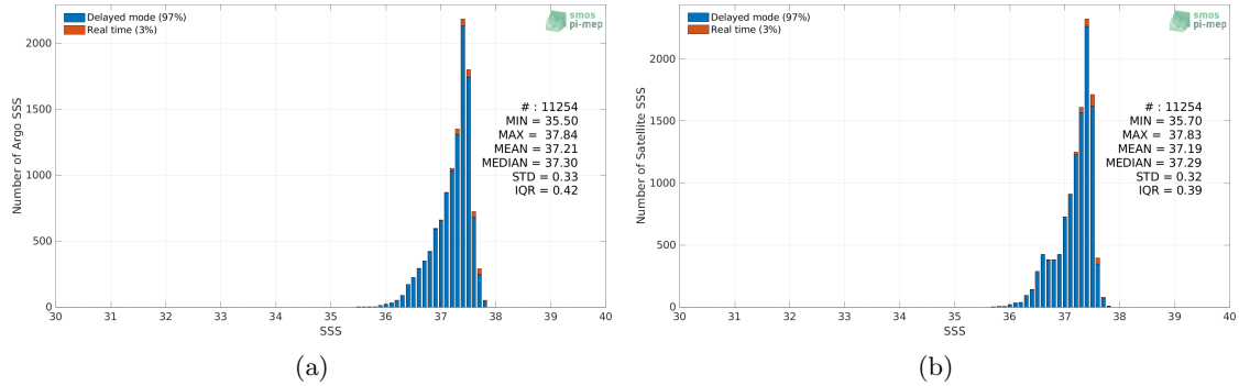
Figure 2: Histograms of SSS from Argo (a) and CCI SSS L4 Merged-OI v3.2 - 30-day running (ESA) (b) considering all match-up pairs per bins of 0.1 over the SPURS 1 Pi-MEP region and for the full satellite product period.
