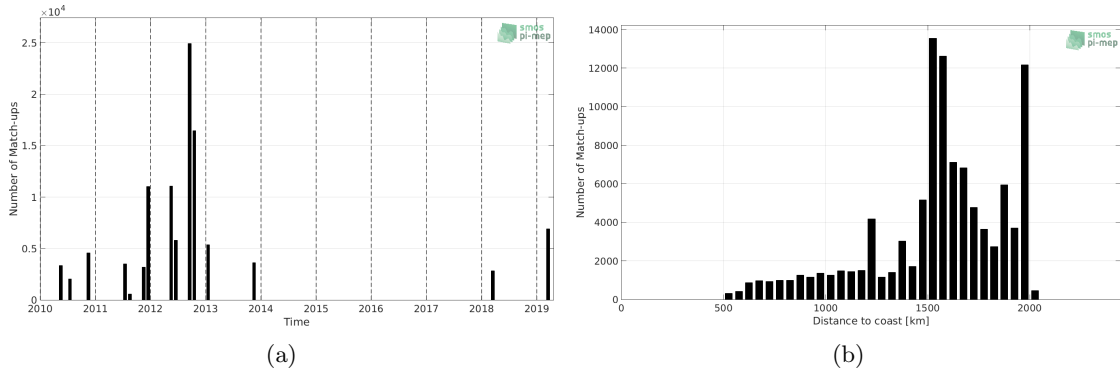
Figure 1: Number of match-ups between TSG (SAMOS) and CCI L4 Merged-OI v2.31 - 7-day running (ESA) SSS as a function of time (a) and as function of the distance to coast (b) over the SPURS 1 Pi-MEP region and for the full satellite product period.
