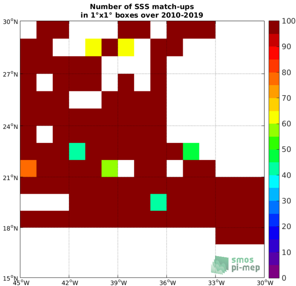
Figure 4: Number of SSS match-ups between TSG (SAMOS) SSS and the CCI L4 Merged-OI v2.31 - 7-day running (ESA) SSS product for the SPURS 1 Pi-MEP region over 1°x1° boxes and for the full satellite product period.
