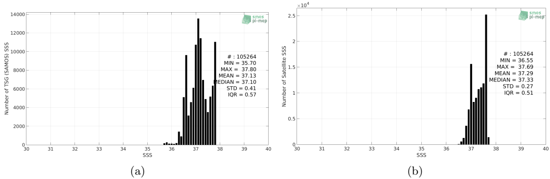
Figure 2: Histograms of SSS from TSG (SAMOS) (a) and CCI L4 Merged-OI v2.31 - 7-day running (ESA) (b) considering all match-up pairs per bins of 0.1 over the SPURS 1 Pi-MEP region and for the full satellite product period.
