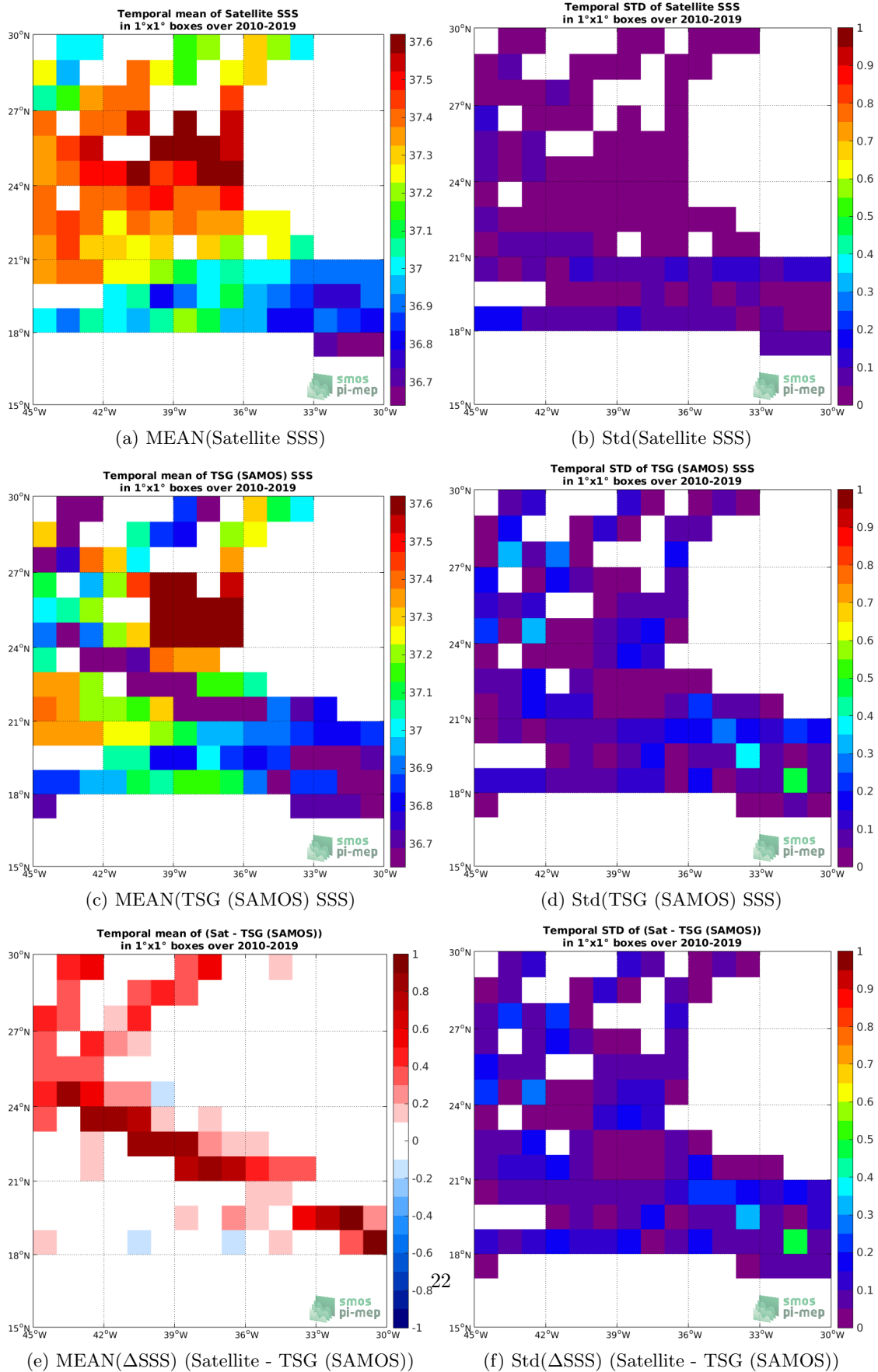
Figure 6: Temporal mean (left) and Std (right) of SSS from CCI L4 Merged-OI v2.31 - 7-day running (ESA) (top), TSG (SAMOS) (middle), and of \Delta SSS (Satellite - TSG (SAMOS)). Only match-up pairs are used to generate these maps.
