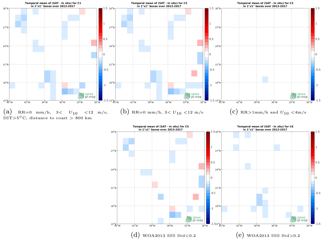
Figure 12: Temporal mean gridded over spatial boxes of size 1^\circ \times 1^\circ of \Delta\text{SSS} (CCI SSS L4 Merged-OI v2.31 - 7-day running (ESA) - TSG (GOSUD-Sailing-ship)) for 5 different subdatasets corresponding to: RR=0 mm/h, 3 < U_{10} < 12 m/s, SST > 5^\circ\text{C} , distance to coast > 800 km (a), RR=0 mm/h, 3 < U_{10} < 12 m/s (b), RR > 1 mm/h and U_{10} < 4 m/s (c), WOA2013 SSS Std < 0.2 (d), WOA2013 SSS Std > 0.2 (e).
