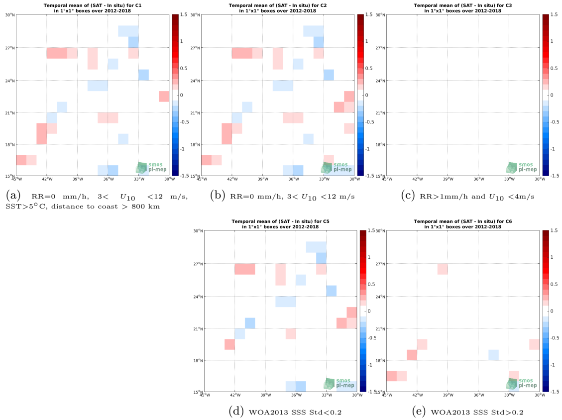
Figure 12: Temporal mean gridded over spatial boxes of size 1°x1° of \Delta SSS (CCI SSS L4 Merged-OI v2.31 - 7-day running (ESA) - TSG (GOSUD-Research-vessel)) for 5 different subdatasets corresponding to:RR=0 mm/h, 3 < U_{10} < 12 m/s, SST>5°C, distance to coast > 800 km (a), RR=0 mm/h, 3 < U_{10} < 12 m/s (b), RR>1mm/h and U_{10} < 4 m/s (c), WOA2013 SSS Std<0.2 (d), WOA2013 SSS Std>0.2 (e).
