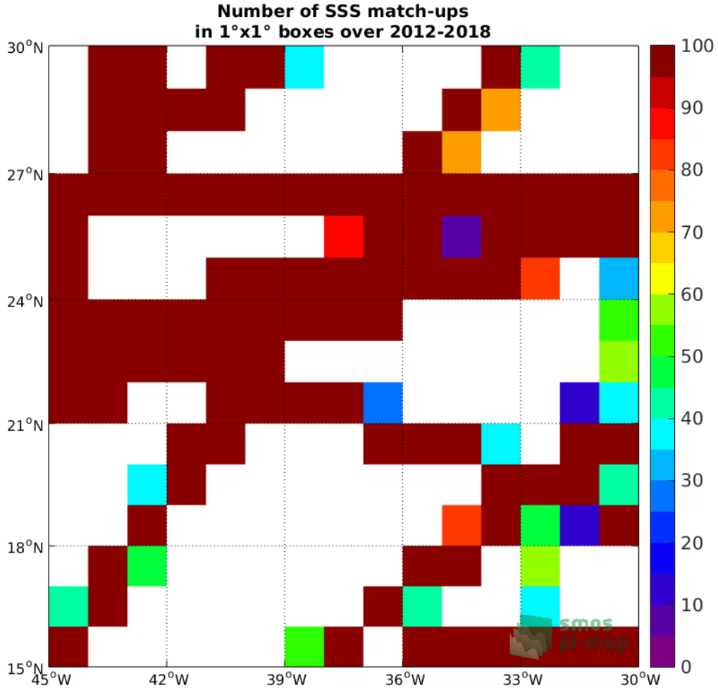
Figure 4: Number of SSS match-ups between TSG (GOSUD-Research-vessel) SSS and the CCI SSS L4 Merged-OI v2.31 - 7-day running (ESA) SSS product for the SPURS 1 Pi-MEP region over 1°x1° boxes and for the full satellite product period.
