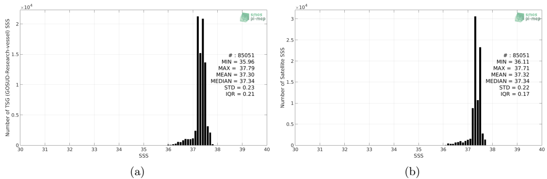
Figure 2: Histograms of SSS from TSG (GOSUD-Research-vessel) (a) and CCI SSS L4 Merged-OI v2.31 - 7-day running (ESA) (b) considering all match-up pairs per bins of 0.1 over the SPURS 1 Pi-MEP region and for the full satellite product period.
