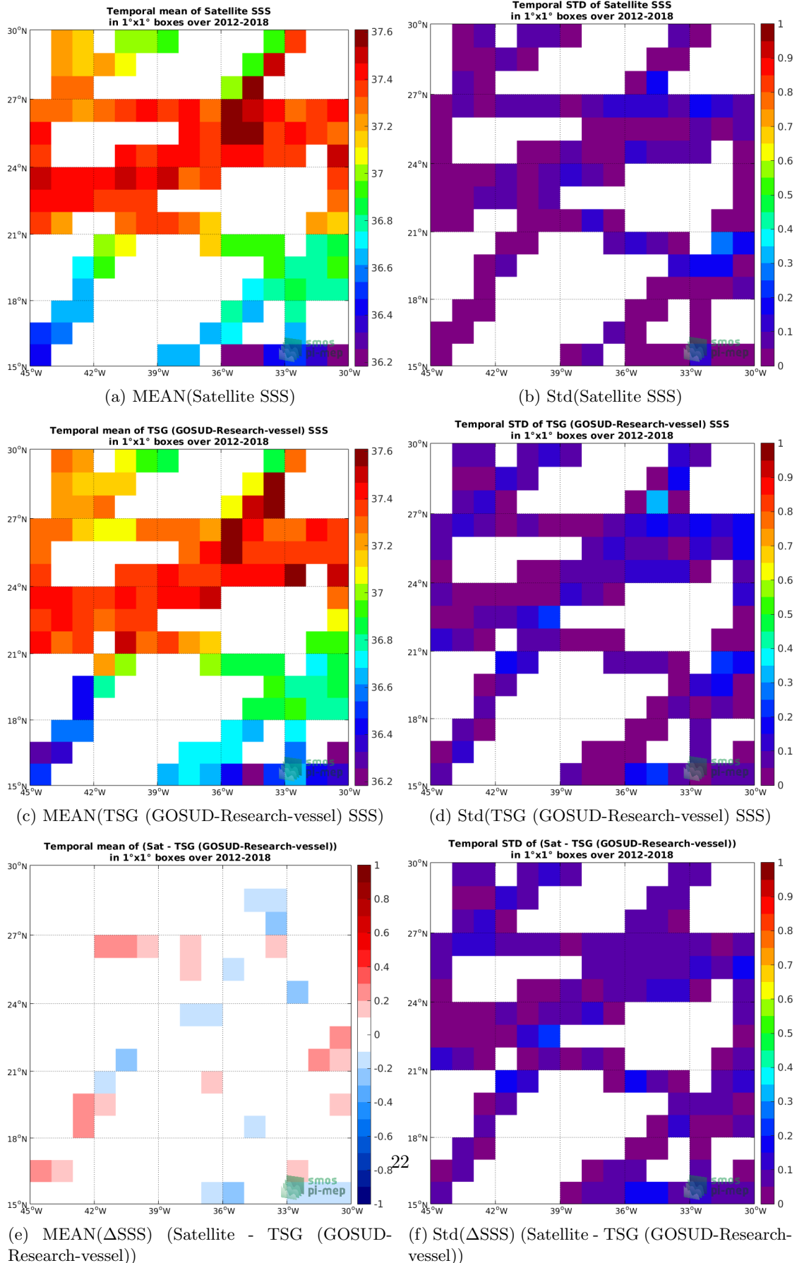
Figure 6: Temporal mean (left) and Std (right) of SSS from CCI SSS L4 Merged-OI v2.31 - 7-day running (ESA) (top), TSG (GOSUD-Research-vessel) (middle), and of \Delta SSS (Satellite - TSG (GOSUD-Research-vessel)). Only match-up pairs are used to generate these maps.
