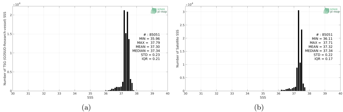
Figure 2: Histograms of SSS from TSG (GOSUD-Research-vessel) (a) and CCI L4 Merged-OI v2.31 - 7-day running (ESA) (b) considering all match-up pairs per bins of 0.1 over the SPURS 1 Pi-MEP region and for the full satellite product period.
