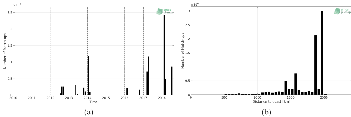
Figure 1: Number of match-ups between TSG (GOSUD-Research-vessel) and CCI L4 Merged-OI v2.31 - 7-day running (ESA) SSS as a function of time (a) and as function of the distance to coast (b) over the SPURS 1 Pi-MEP region and for the full satellite product period.
