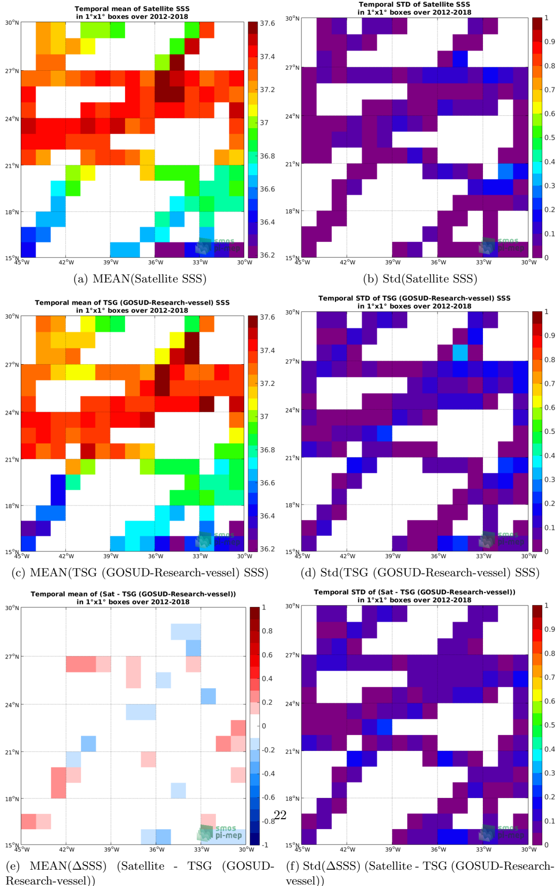
Figure 6: Temporal mean (left) and Std (right) of SSS from CCI L4 Merged-OI v2.31 - 7-day running (ESA) (top), TSG (GOSUD-Research-vessel) (middle), and of \Delta SSS (Satellite - TSG (GOSUD-Research-vessel)). Only match-up pairs are used to generate these maps.
