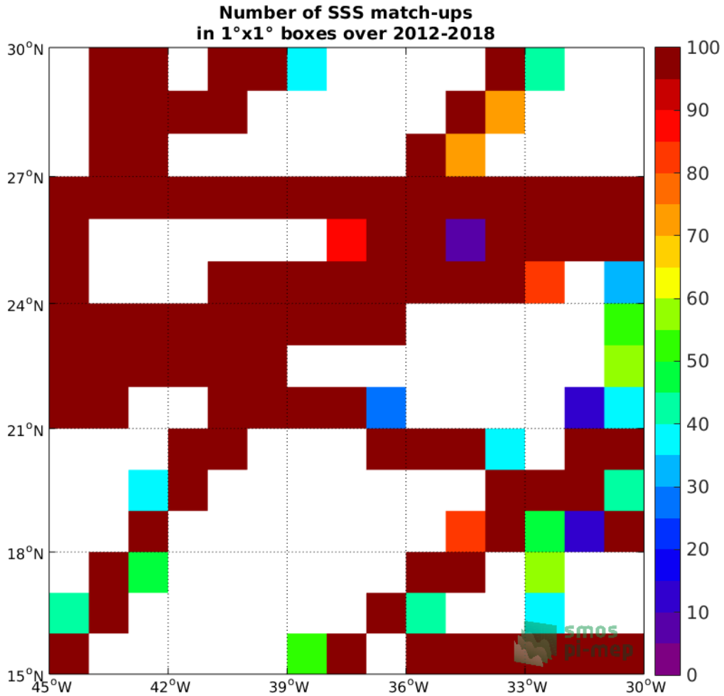
Figure 4: Number of SSS match-ups between TSG (GOSUD-Research-vessel) SSS and the CCI L4 Merged-OI v2.31 - 7-day running (ESA) SSS product for the SPURS 1 Pi-MEP region over 1°x1° boxes and for the full satellite product period.
