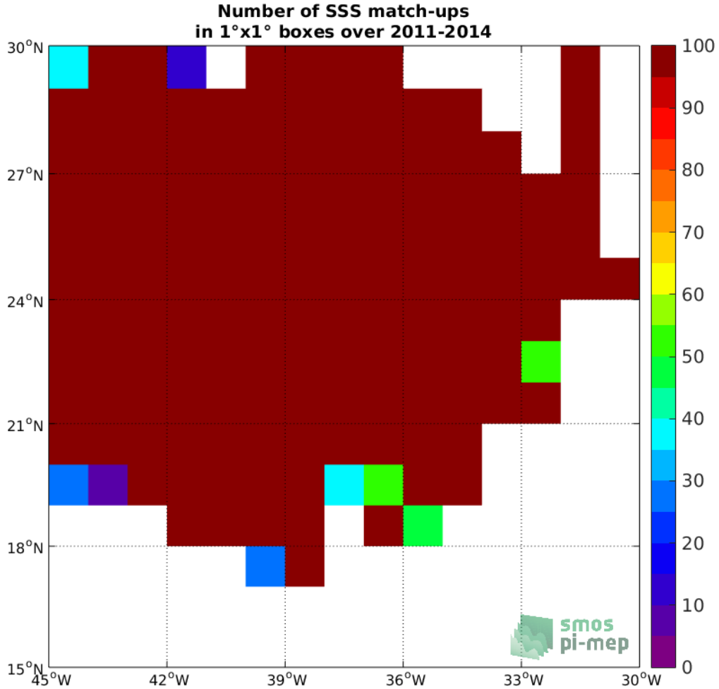
Figure 3: Number of SSS match-ups between Surface drifters SSS and the CCI SSS L4 Merged-OI v2.31 - 7-day running (ESA) SSS product for the SPURS 1 Pi-MEP region over 1°x1° boxes and for the full satellite product period.
