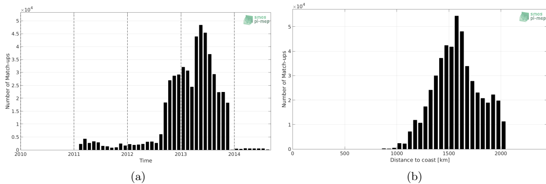
Figure 1: Number of match-ups between Surface drifters and CCI SSS L4 Merged-OI v2.31 - 7-day running (ESA) SSS as a function of time (a) and as function of the distance to coast (b) over the SPURS 1 Pi-MEP region and for the full satellite product period.
