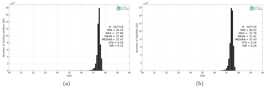
Figure 2: Histograms of SSS from Surface drifters (a) and CCI SSS L4 Merged-OI v2.31 - 7-day running (ESA) (b) considering all match-up pairs per bins of 0.1 over the SPURS 1 Pi-MEP region and for the full satellite product period.
