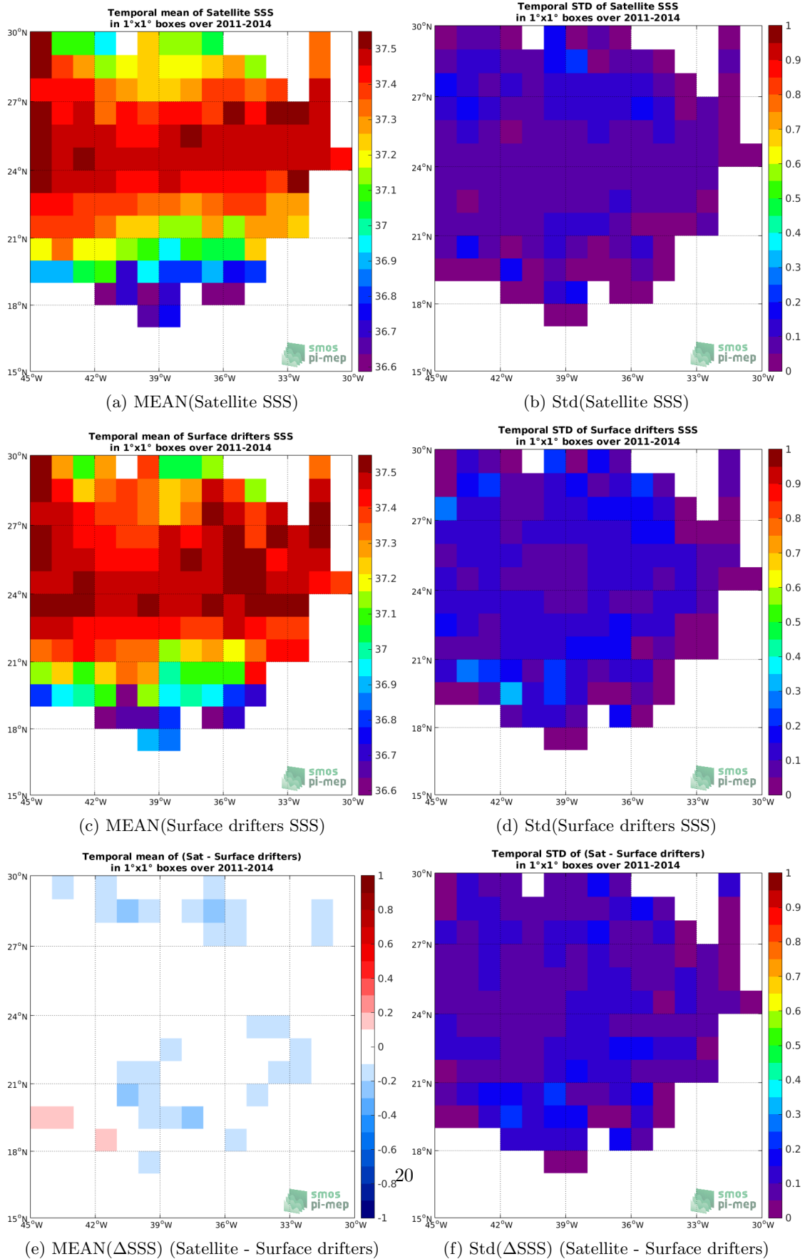
Figure 5: Temporal mean (left) and Std (right) of SSS from CCI SSS L4 Merged-OI v2.31 - 7-day running (ESA) (top), Surface drifters (middle), and of \Delta SSS (Satellite - Surface drifters). Only match-up pairs are used to generate these maps.
