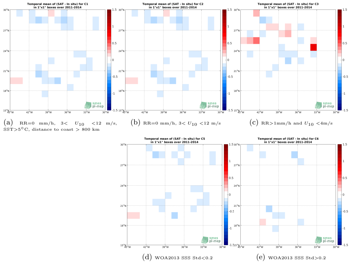
Figure 11: Temporal mean gridded over spatial boxes of size 1^\circ \times 1^\circ of \Delta SSS (CCI SSS L4 Merged-OI v2.31 - 7-day running (ESA) - Surface drifters) for 5 different subdatasets corresponding to:RR=0 mm/h, 3 < U_{10} < 12 m/s, SST >5^\circ C, distance to coast > 800 km (a), RR=0 mm/h, 3 < U_{10} < 12 m/s (b), RR >1 mm/h and U_{10} < 4 m/s (c), WOA2013 SSS Std <0.2 (d), WOA2013 SSS Std >0.2 (e).
