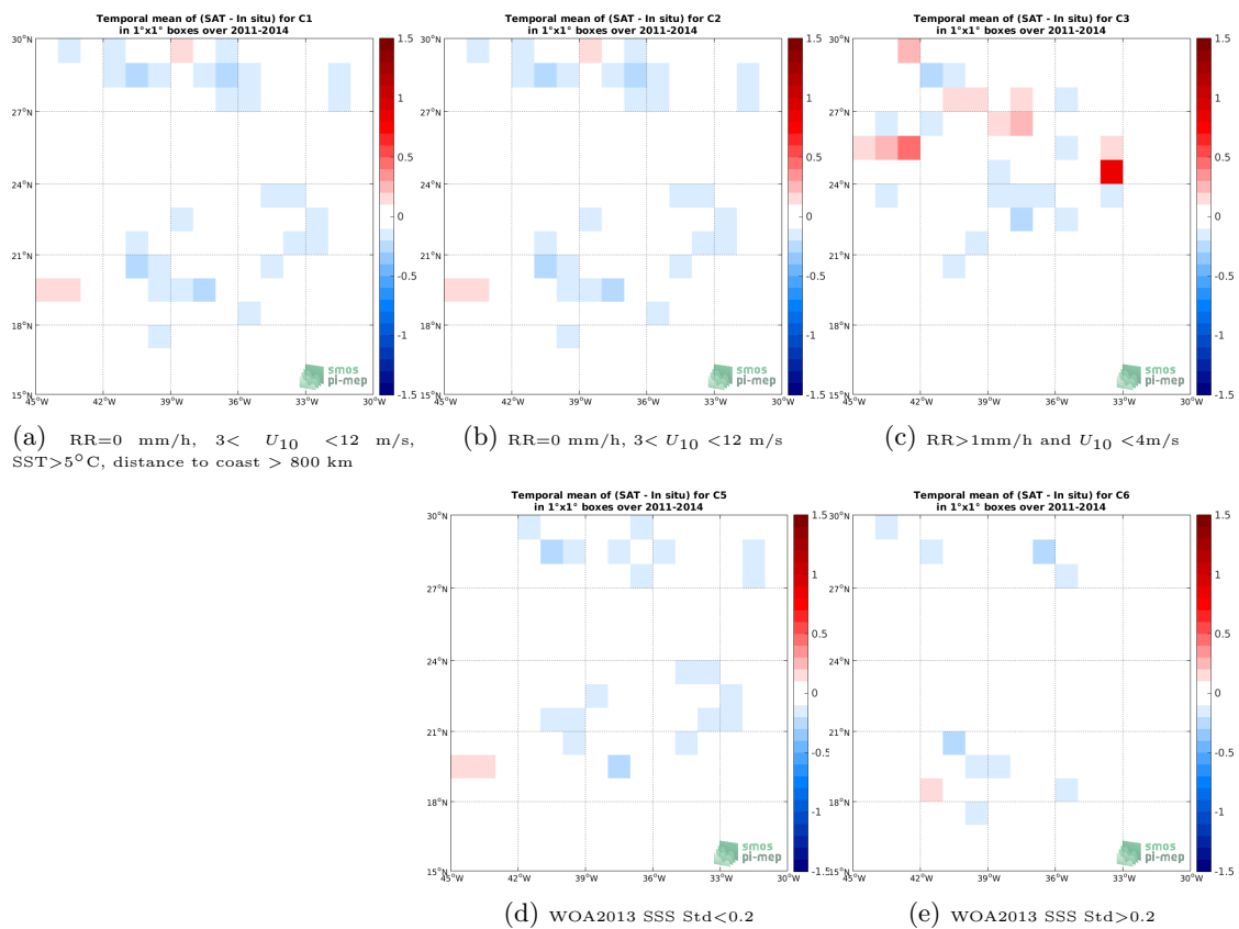
Figure 11: Temporal mean gridded over spatial boxes of size 1^\circ \times 1^\circ of \Delta SSS (CCI L4 Merged-OI v2.31 - 7-day running (ESA) - Surface drifters) for 5 different subdatasets corresponding to:RR=0 mm/h, 3 < U_{10} < 12 m/s, SST >5^\circ C, distance to coast > 800 km (a), RR=0 mm/h, 3 < U_{10} < 12 m/s (b), RR >1 mm/h and U_{10} < 4 m/s (c), WOA2013 SSS Std <0.2 (d), WOA2013 SSS Std >0.2 (e).
