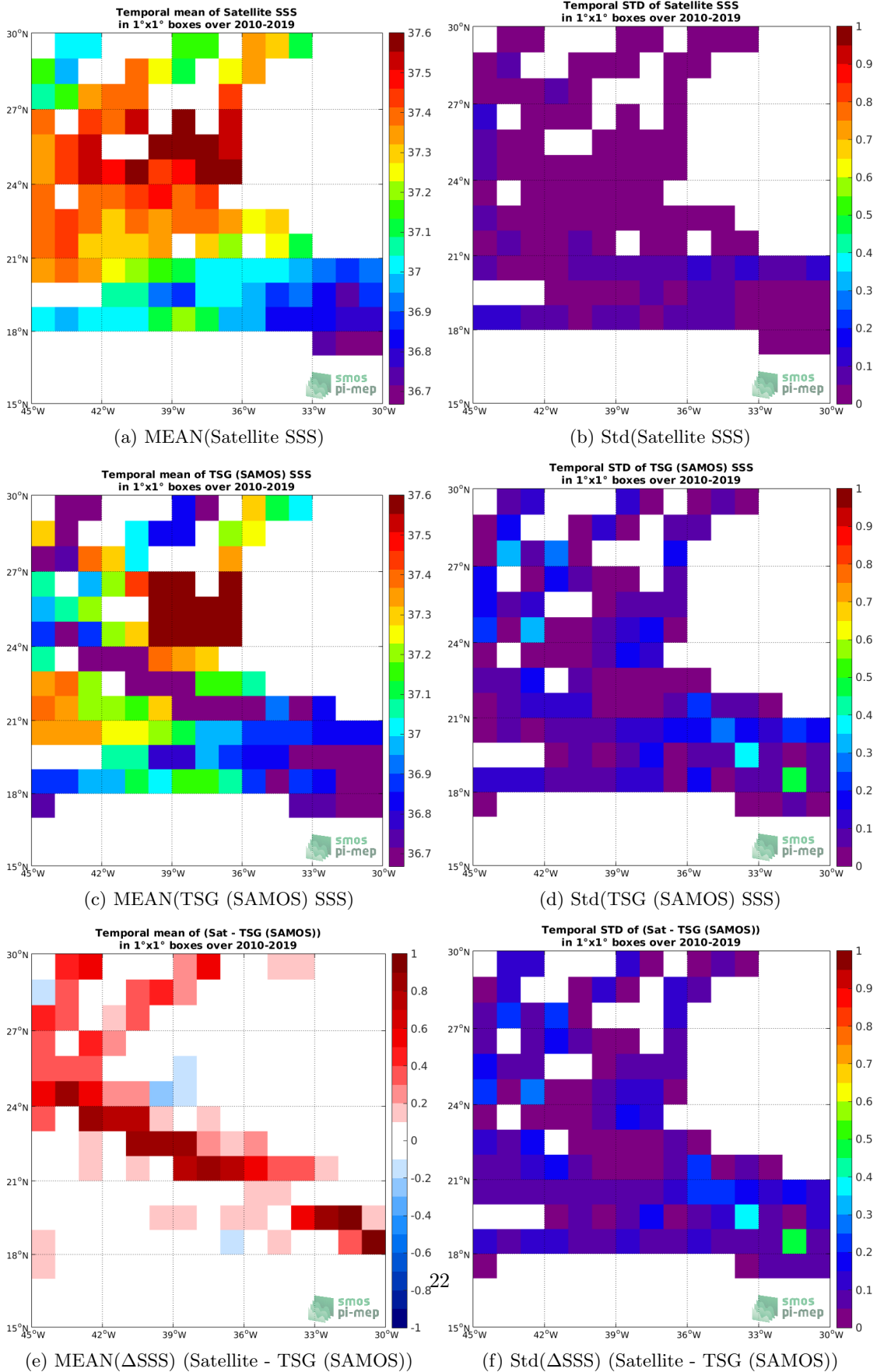
Figure 6: Temporal mean (left) and Std (right) of SSS from CCI SSS L4 Merged-OI v2.31 - 30-day running (ESA) (top), TSG (SAMOS) (middle), and of \Delta SSS (Satellite - TSG (SAMOS)). Only match-up pairs are used to generate these maps.
