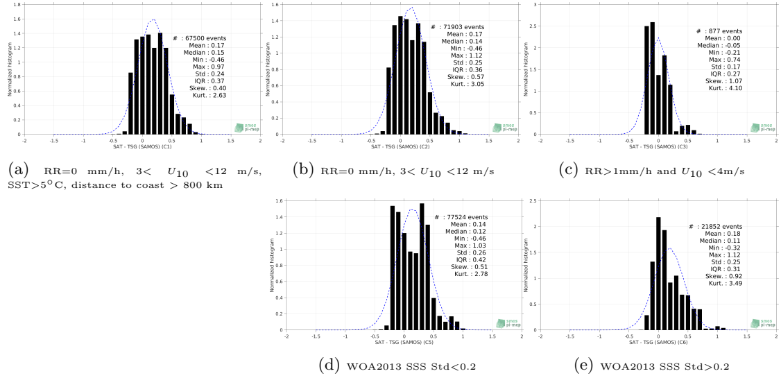
Figure 13: Normalized histogram of \Delta SSS (CCI SSS L4 Merged-OI v2.31 - 30-day running (ESA) - TSG (SAMOS)) for 5 different subdatasets corresponding to: RR=0 mm/h, 3 < U_{10} < 12 m/s, SST > 5°C, distance to coast > 800 km (a), RR=0 mm/h, 3 < U_{10} < 12 m/s (b), RR > 1mm/h and U_{10} < 4 m/s (c), WOA2013 SSS Std < 0.2 (d), WOA2013 SSS Std > 0.2 (e).
