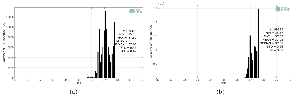
Figure 2: Histograms of SSS from TSG (SAMOS) (a) and CCI L4 Merged-OI v2.31 - 30-day running (ESA) (b) considering all match-up pairs per bins of 0.1 over the SPURS 1 Pi-MEP region and for the full satellite product period.
