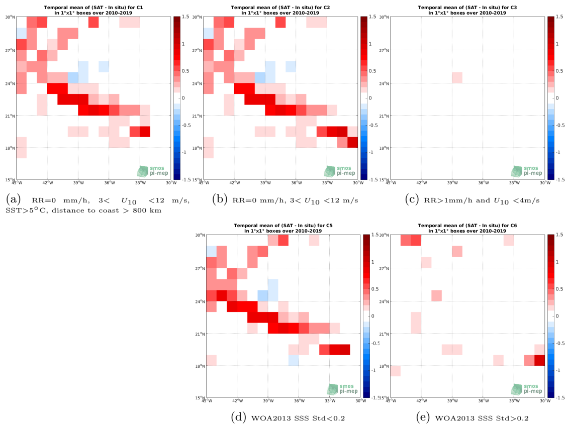
Figure 12: Temporal mean gridded over spatial boxes of size 1^\circ \times 1^\circ of \Delta\text{SSS} (CCI L4 Merged-OI v2.31 - 30-day running (ESA) - TSG (SAMOS)) for 5 different subdatasets corresponding to:RR=0 mm/h, 3 < U_{10} < 12 m/s, SST >5^\circ\text{C} , distance to coast > 800 km (a), RR=0 mm/h, 3 < U_{10} < 12 m/s (b), RR >1 mm/h and U_{10} < 4 m/s (c), WOA2013 SSS Std <0.2 (d), WOA2013 SSS Std >0.2 (e).
