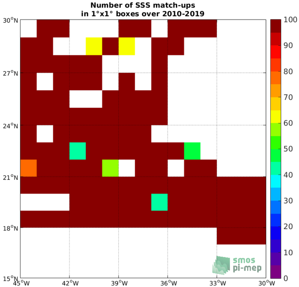
Figure 4: Number of SSS match-ups between TSG (SAMOS) SSS and the CCI L4 Merged-OI v2.31 - 30-day running (ESA) SSS product for the SPURS 1 Pi-MEP region over 1°x1° boxes and for the full satellite product period.
