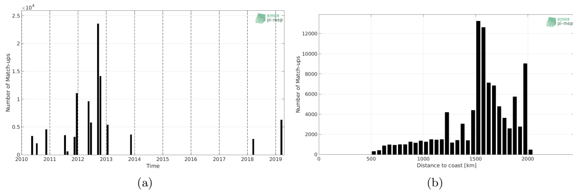
Figure 1: Number of match-ups between TSG (SAMOS) and CCI L4 Merged-OI v2.31 - 30-day running (ESA) SSS as a function of time (a) and as function of the distance to coast (b) over the SPURS 1 Pi-MEP region and for the full satellite product period.
