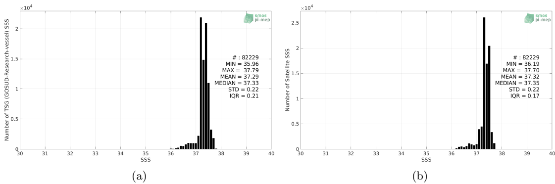
Figure 2: Histograms of SSS from TSG (GOSUD-Research-vessel) (a) and CCI SSS L4 Merged-OI v2.31 - 30-day running (ESA) (b) considering all match-up pairs per bins of 0.1 over the SPURS 1 Pi-MEP region and for the full satellite product period.
