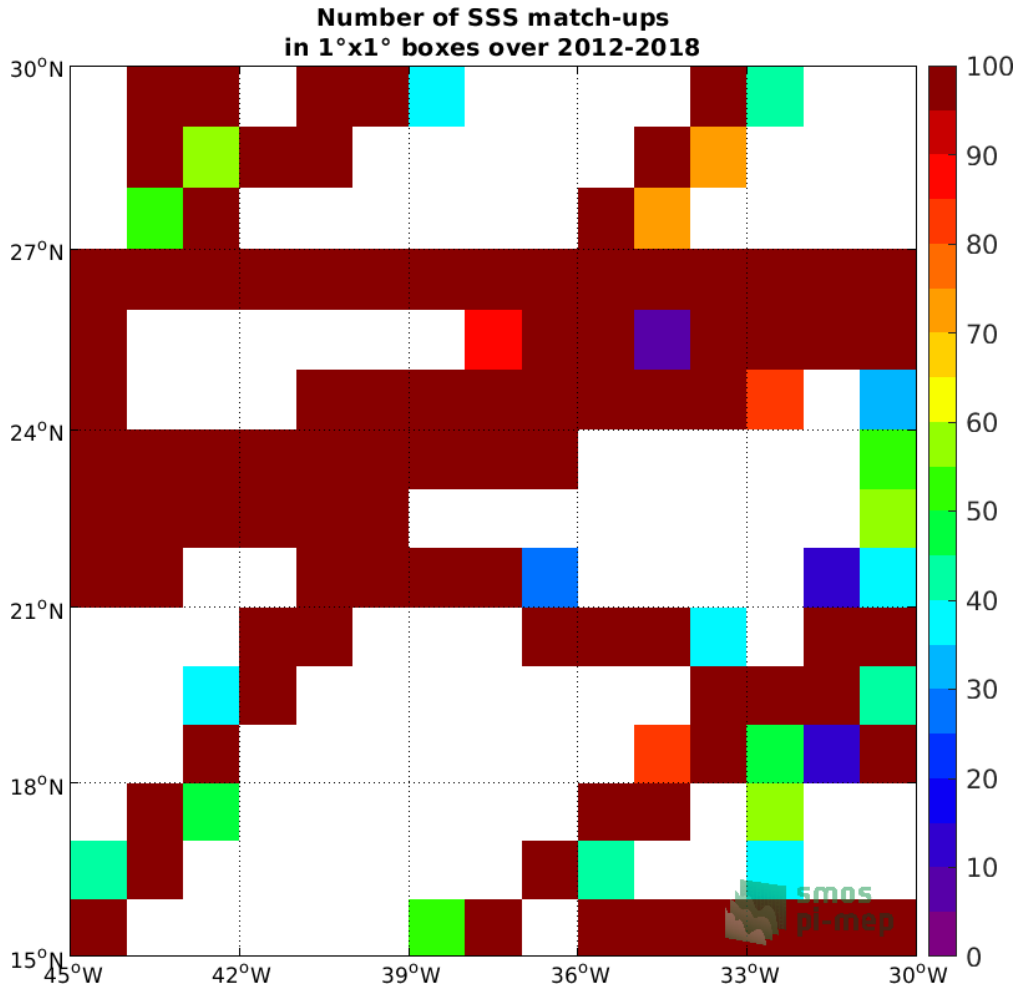
Figure 4: Number of SSS match-ups between TSG (GOSUD-Research-vessel) SSS and the CCI SSS L4 Merged-OI v2.31 - 30-day running (ESA) SSS product for the SPURS 1 Pi-MEP region over 1°x1° boxes and for the full satellite product period.
