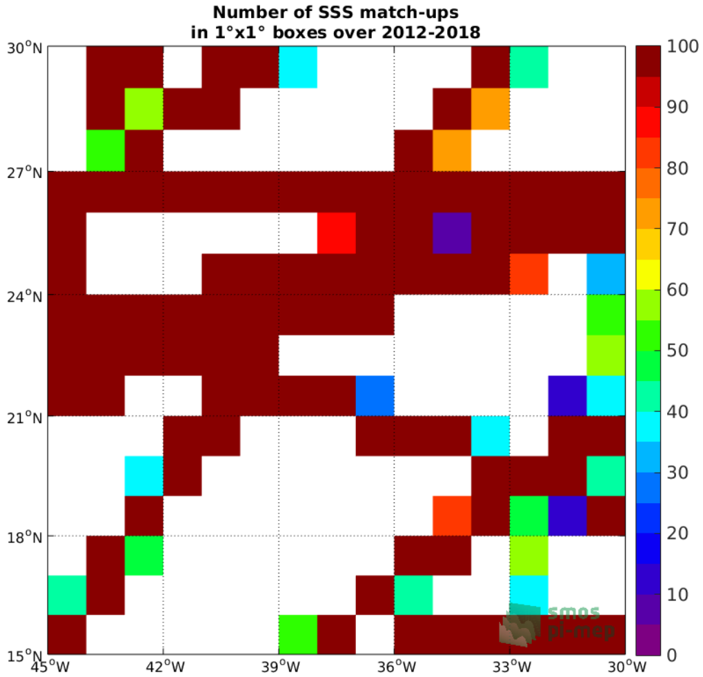
Figure 4: Number of SSS match-ups between TSG (GOSUD-Research-vessel) SSS and the CCI L4 Merged-OI v2.31 - 30-day running (ESA) SSS product for the SPURS 1 Pi-MEP region over 1°x1° boxes and for the full satellite product period.
