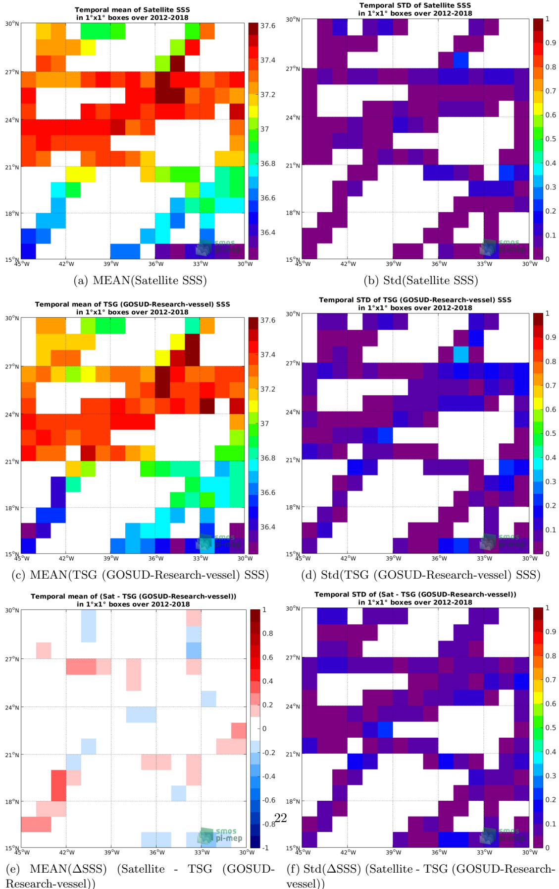
Figure 6: Temporal mean (left) and Std (right) of SSS from CCI L4 Merged-OI v2.31 - 30-day running (ESA) (top), TSG (GOSUD-Research-vessel) (middle), and of \Delta SSS (Satellite - TSG (GOSUD-Research-vessel)). Only match-up pairs are used to generate these maps.
