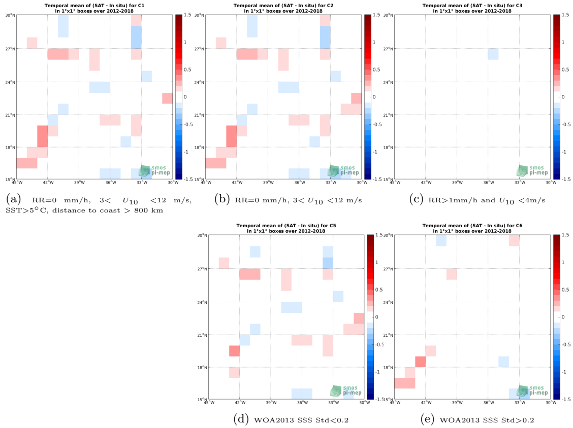
Figure 12: Temporal mean gridded over spatial boxes of size 1^\circ \times 1^\circ of \Delta SSS (CCI L4 Merged-OI v2.31 - 30-day running (ESA) - TSG (GOSUD-Research-vessel)) for 5 different subdatasets corresponding to: RR=0 mm/h, 3 < U_{10} < 12 m/s, SST>5°C, distance to coast > 800 km (a), RR=0 mm/h, 3 < U_{10} < 12 m/s (b), RR>1mm/h and U_{10} < 4 m/s (c), WOA2013 SSS Std<0.2 (d), WOA2013 SSS Std>0.2 (e).
