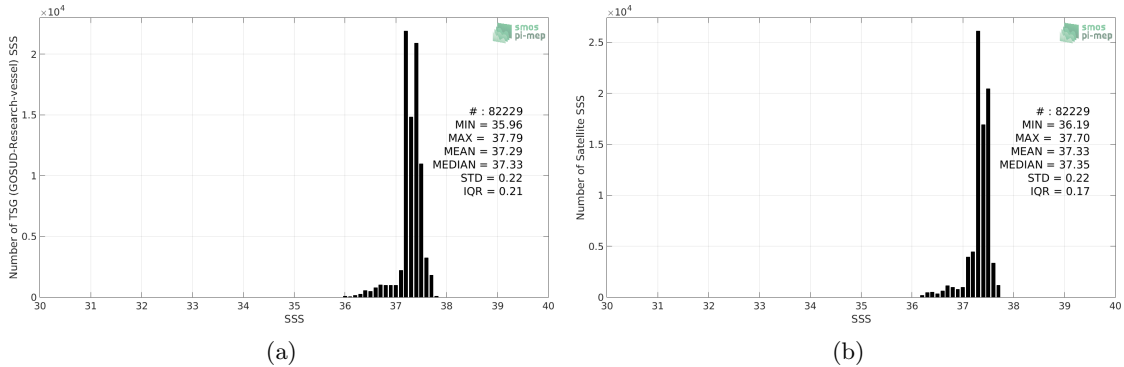
Figure 2: Histograms of SSS from TSG (GOSUD-Research-vessel) (a) and CCI L4 Merged-OI v2.31 - 30-day running (ESA) (b) considering all match-up pairs per bins of 0.1 over the SPURS 1 Pi-MEP region and for the full satellite product period.
