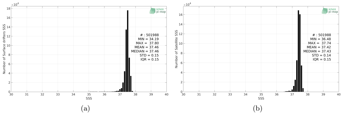
Figure 2: Histograms of SSS from Surface drifters (a) and CCI SSS L4 Merged-OI v2.31 - 30-day running (ESA) (b) considering all match-up pairs per bins of 0.1 over the SPURS 1 Pi-MEP region and for the full satellite product period.
