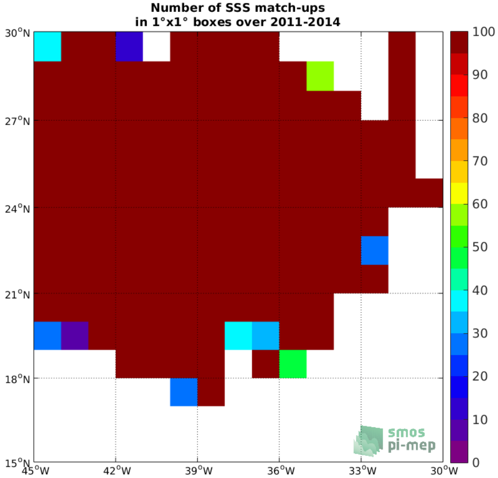
Figure 3: Number of SSS match-ups between Surface drifters SSS and the CCI SSS L4 Merged-OI v2.31 - 30-day running (ESA) SSS product for the SPURS 1 Pi-MEP region over 1°x1° boxes and for the full satellite product period.
