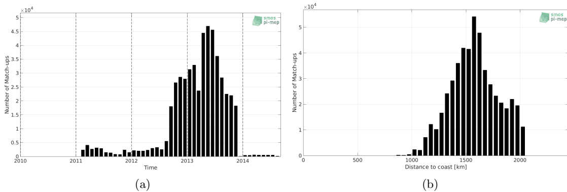
Figure 1: Number of match-ups between Surface drifters and CCI SSS L4 Merged-OI v2.31 - 30-day running (ESA) SSS as a function of time (a) and as function of the distance to coast (b) over the SPURS 1 Pi-MEP region and for the full satellite product period.
