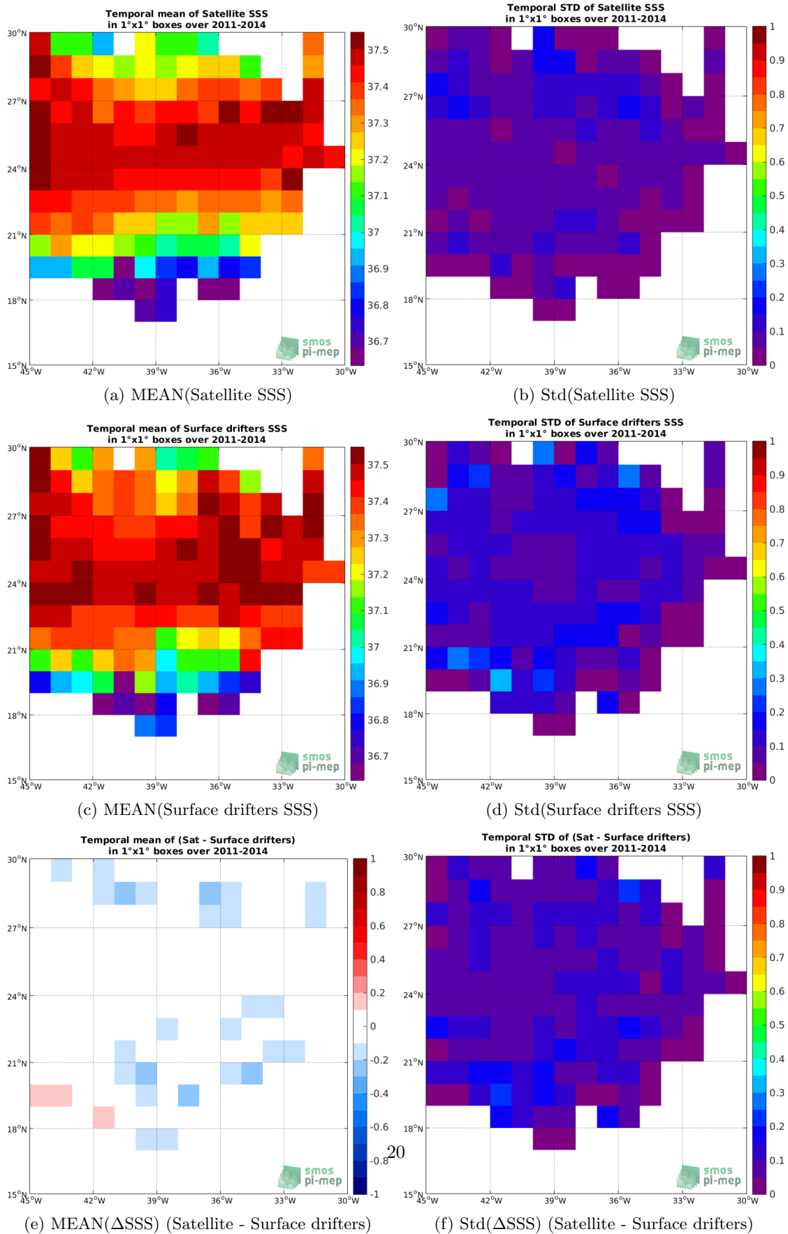
Figure 5: Temporal mean (left) and Std (right) of SSS from CCI SSS L4 Merged-OI v2.31 - 30-day running (ESA) (top), Surface drifters (middle), and of \Delta SSS (Satellite - Surface drifters). Only match-up pairs are used to generate these maps.
