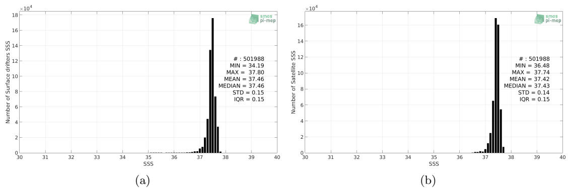
Figure 2: Histograms of SSS from Surface drifters (a) and CCI L4 Merged-OI v2.31 - 30-day running (ESA) (b) considering all match-up pairs per bins of 0.1 over the SPURS 1 Pi-MEP region and for the full satellite product period.
