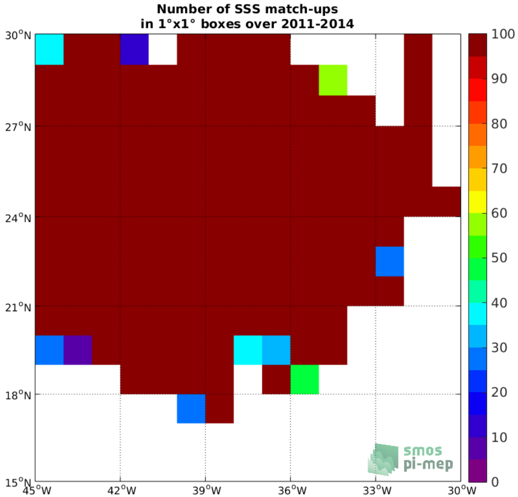
Figure 3: Number of SSS match-ups between Surface drifters SSS and the CCI L4 Merged-OI v2.31 - 30-day running (ESA) SSS product for the SPURS 1 Pi-MEP region over 1°x1° boxes and for the full satellite product period.
