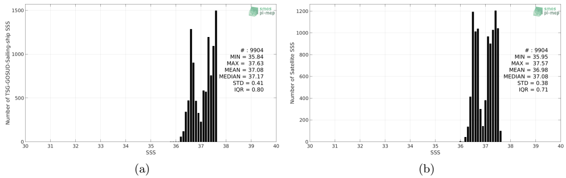
Figure 2: Histograms of SSS from TSG-GOSUD-Sailing-ship (a) and CCI-L4-ESA-MERGED-OI-V1.8-30DAY-RUNNING (b) considering all match-up pairs per bins of 0.1 over the SPURS 1 Pi-MEP region and for the full satellite product period.
