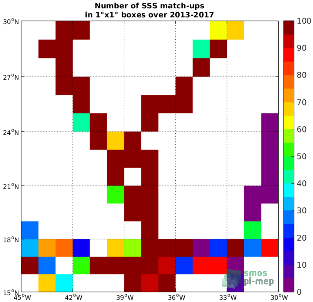
Figure 4: Number of SSS match-ups between TSG-GOSUD-Sailing-ship SSS and the CCI-L4-ESA-MERGED-OI-V1.8-30DAY-RUNNING SSS product for the SPURS 1 Pi-MEP region over 1°x1° boxes and for the full satellite product period.
