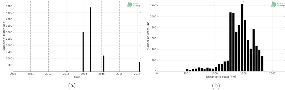
Figure 1: Number of match-ups between TSG-GOSUD-Sailing-ship and CCI-L4-ESA-MERGED-OI-V1.8-30DAY-RUNNING SSS as a function of time (a) and as function of the distance to coast (b) over the SPURS 1 Pi-MEP region and for the full satellite product period.
