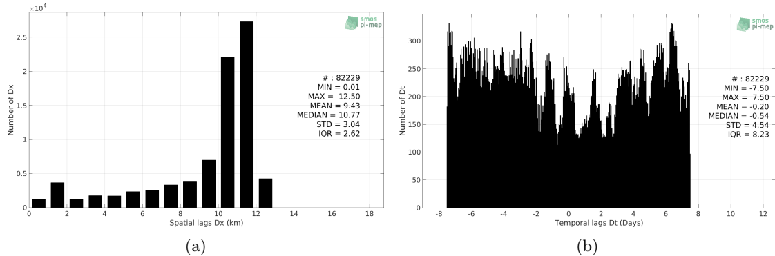
Figure 5: Histograms of the spatial (a) and temporal (b) lags between the time of the TSG-GOSUD-Research-vessel measurements and the date of the corresponding CCI-L4-ESA-MERGED-OI-V1.8-30DAY-RUNNING SSS product.
