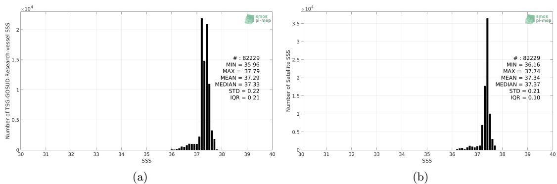
Figure 2: Histograms of SSS from TSG-GOSUD-Research-vessel (a) and CCI-L4-ESA-MERGED-OI-V1.8-30DAY-RUNNING (b) considering all match-up pairs per bins of 0.1 over the SPURS 1 Pi-MEP region and for the full satellite product period.
