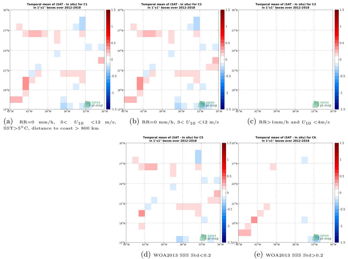
Figure 12: Temporal mean gridded over spatial boxes of size 1^\circ \times 1^\circ of \Delta SSS (CCI-L4-ESA-MERGED-OI-V1.8-30DAY-RUNNING - TSG-GOSUD-Research-vessel) for 5 different sub-datasets corresponding to:RR=0 mm/h, 3 < U_{10} < 12 m/s, SST >5^\circ C, distance to coast > 800 km (a), RR=0 mm/h, 3 < U_{10} < 12 m/s (b), RR >1 mm/h and U_{10} < 4 m/s (c), WOA2013 SSS Std <0.2 (d), WOA2013 SSS Std >0.2 (e).
