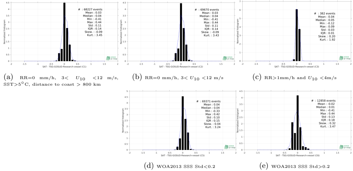
Figure 13: Normalized histogram of \Delta SSS (CCI-L4-ESA-MERGED-OI-V1.8-30DAY-RUNNING - TSG-GOSUD-Research-vessel) for 5 different subdatasets corresponding to: RR=0 mm/h, 3 < U_{10} < 12 m/s, SST > 5°C, distance to coast > 800 km (a), RR=0 mm/h, 3 < U_{10} < 12 m/s (b), RR > 1mm/h and U_{10} < 4 m/s (c), WOA2013 SSS Std < 0.2 (d), WOA2013 SSS Std > 0.2 (e).
