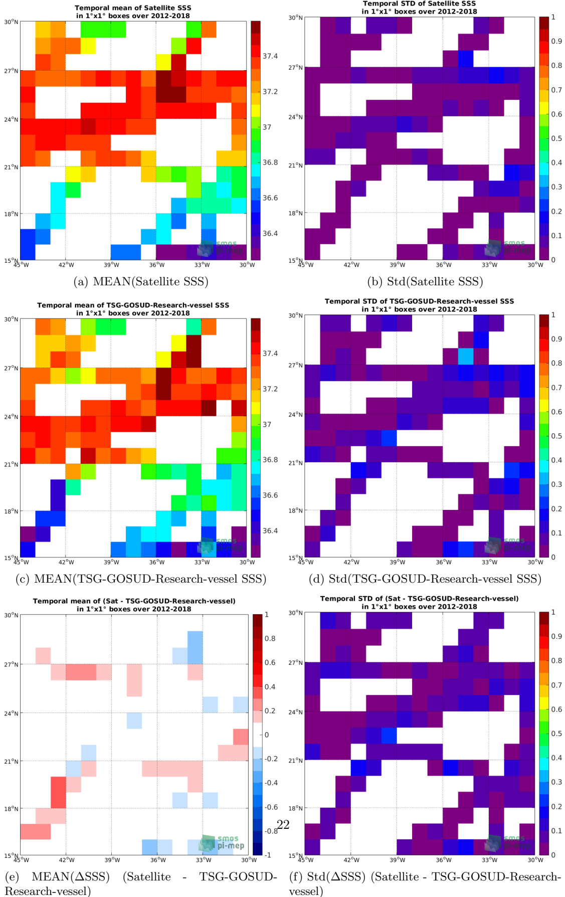
Figure 6: Temporal mean (left) and Std (right) of SSS from CCI-L4-ESA-MERGED-OI-V1.8-30DAY-RUNNING (top), TSG-GOSUD-Research-vessel (middle), and of \Delta SSS (Satellite - TSG-GOSUD-Research-vessel). Only match-up pairs are used to generate these maps.
