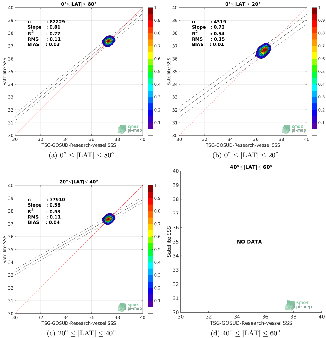
Figure 9: Contour maps of the concentration of CCI-L4-ESA-MERGED-OI-V1.8-30DAY-RUNNING SSS (y-axis) versus TSG-GOSUD-Research-vessel SSS (x-axis) at match-up pairs for different latitude bands. For each plot, the red line shows x=y . The black thin and dashed lines indicate a linear fit through the data cloud and the \pm 95\% confidence levels, respectively. The number match-up pairs n , the slope and R^2 coefficient of the linear fit, the root mean square (RMS) and the mean bias between satellite and in situ data are indicated for each latitude band in each plots.
