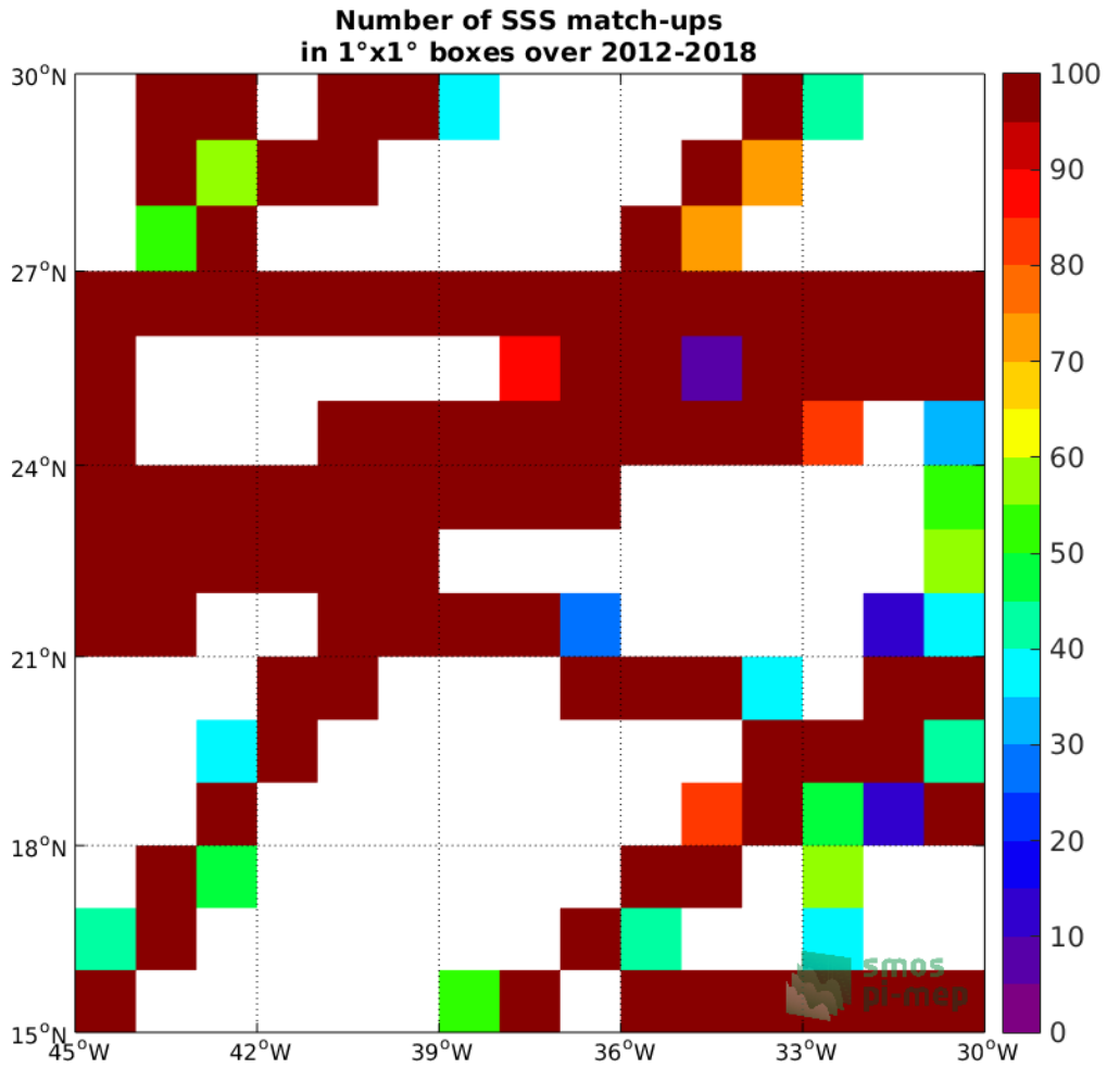
Figure 4: Number of SSS match-ups between TSG-GOSUD-Research-vessel SSS and the CCI-L4-ESA-MERGED-OI-V1.8-30DAY-RUNNING SSS product for the SPURS 1 Pi-MEP region over 1°x1° boxes and for the full satellite product period.
