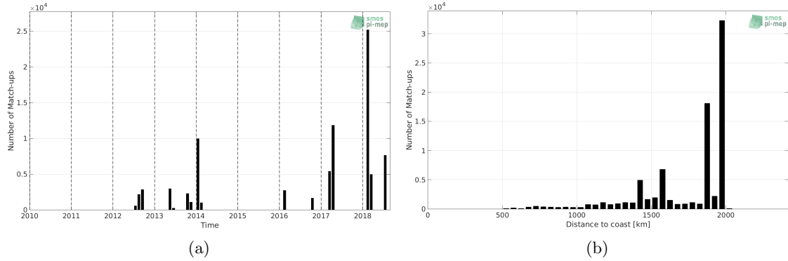
Figure 1: Number of match-ups between TSG-GOSUD-Research-vessel and CCI-L4-ESA-MERGED-OI-V1.8-30DAY-RUNNING SSS as a function of time (a) and as function of the distance to coast (b) over the SPURS 1 Pi-MEP region and for the full satellite product period.
