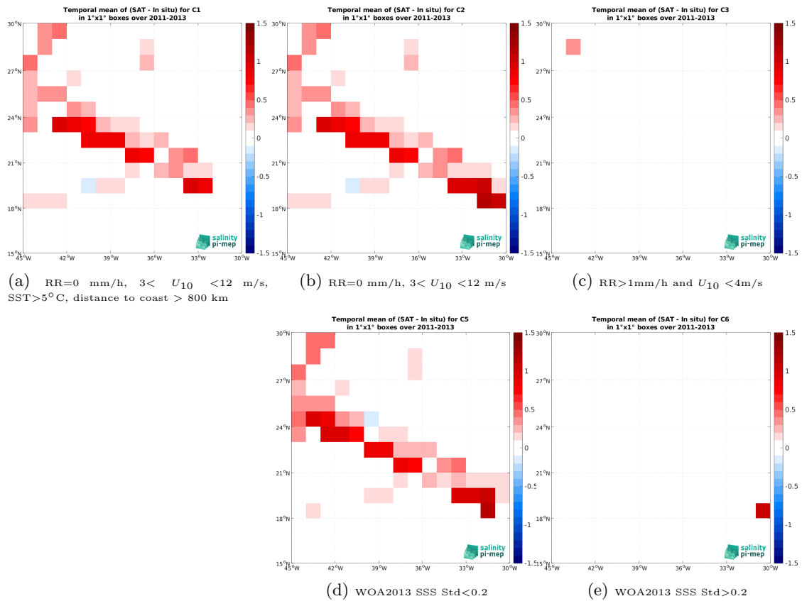
Figure 14: Temporal mean gridded over spatial boxes of size 1^\circ \times 1^\circ of \Delta SSS (Aquarius SSS L4 OI v5 - Weekly (IPRC) - TSG (SAMOS)) for 5 different subdatasets corresponding to: RR=0 mm/h, 3 < U_{10} < 12 m/s, SST > 5^\circ C , distance to coast > 800 km (a), RR=0 mm/h, 3 < U_{10} < 12 m/s (b), RR > 1 mm/h and U_{10} < 4 m/s (c), WOA2013 SSS Std < 0.2 (d), WOA2013 SSS Std > 0.2 (e).
