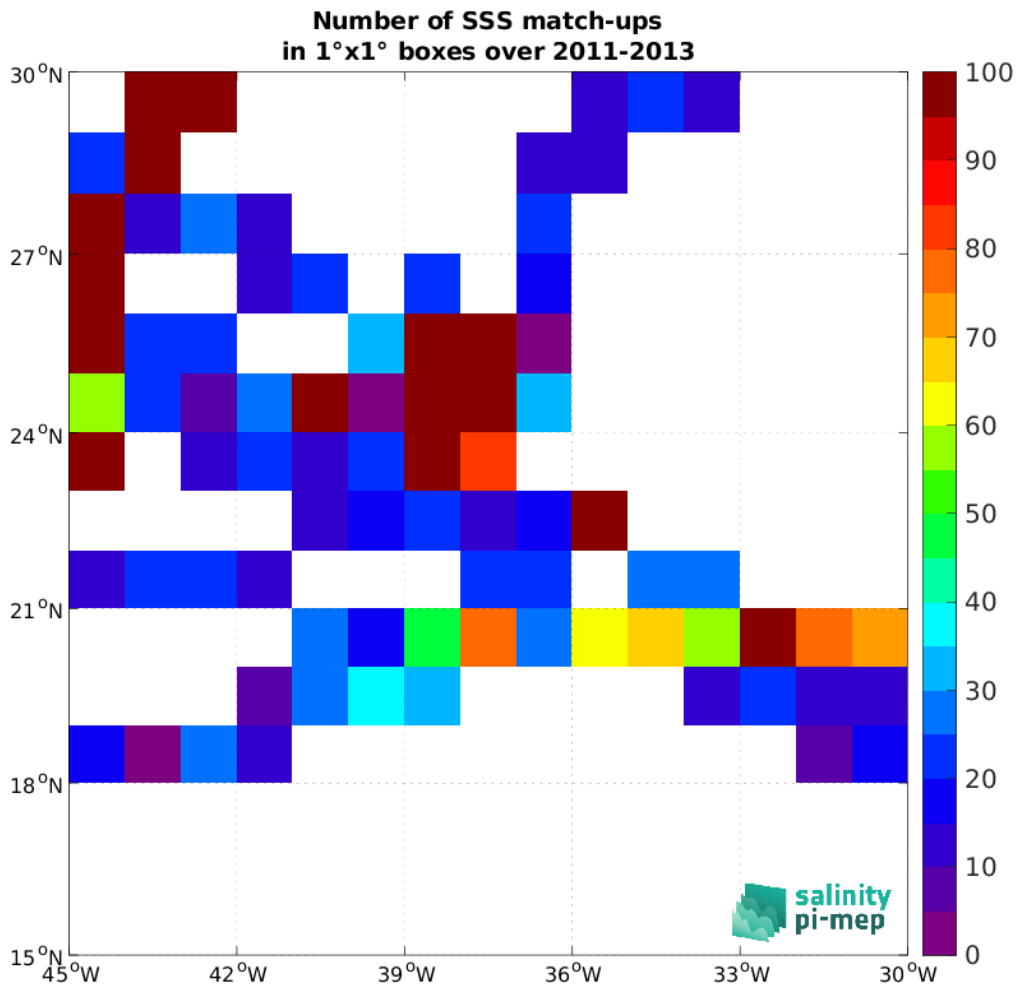
Figure 5: Number of SSS match-ups between TSG (SAMOS) SSS and the Aquarius SSS L4 OI v5 - Weekly (IPRC) SSS product for the SPURS 1 Pi-MEP region over 1°×1° boxes and for the full satellite product period.
