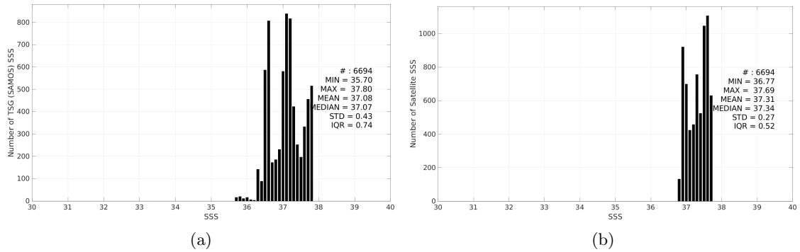
Figure 3: Histograms of SSS from TSG (SAMOS) (a) and Aquarius SSS L4 OI v5 - Weekly (IPRC) (b) considering all match-up pairs per bins of 0.1 over the SPURS 1 Pi-MEP region and for the full satellite product period.
