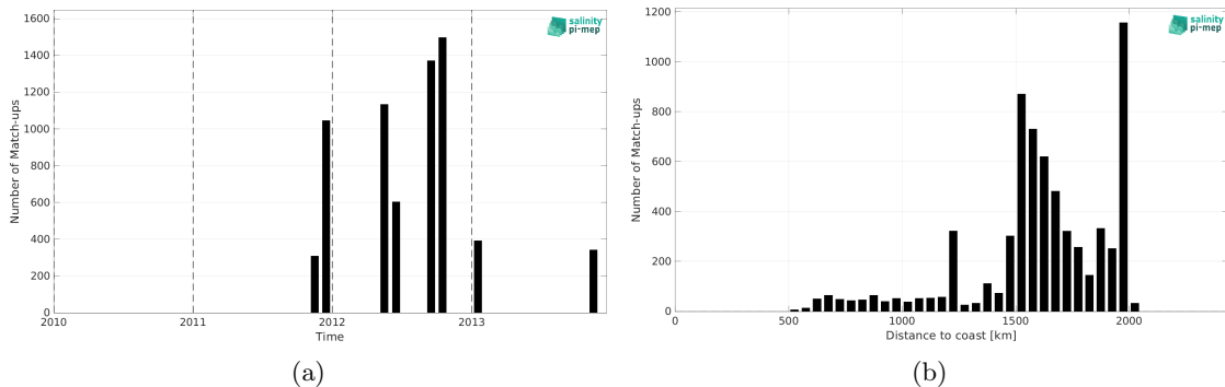
Figure 2: Number of match-ups between TSG (SAMOS) and Aquarius SSS L4 OI v5 - Weekly (IPRC) SSS as a function of time (a) and as function of the distance to coast (b) over the SPURS 1 Pi-MEP region and for the full satellite product period.
