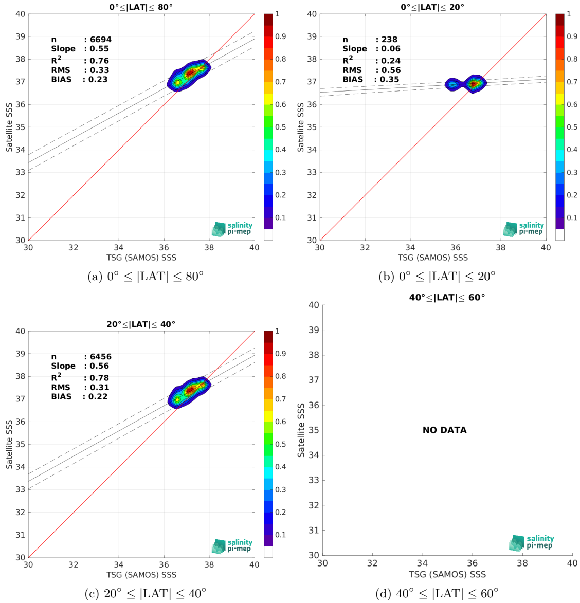
Figure 10: Contour maps of the concentration of Aquarius SSS L4 OI v5 - Weekly (IPRC) SSS (y-axis) versus TSG (SAMOS) SSS (x-axis) at match-up pairs for different latitude bands. For each plot, the red line shows x=y . The black thin and dashed lines indicate a linear fit through the data cloud and the \pm 95\% confidence levels, respectively. The number match-up pairs n , the slope and R^2 coefficient of the linear fit, the root mean square (RMS) and the mean bias between satellite and in situ data are indicated for each latitude band in each plots.
