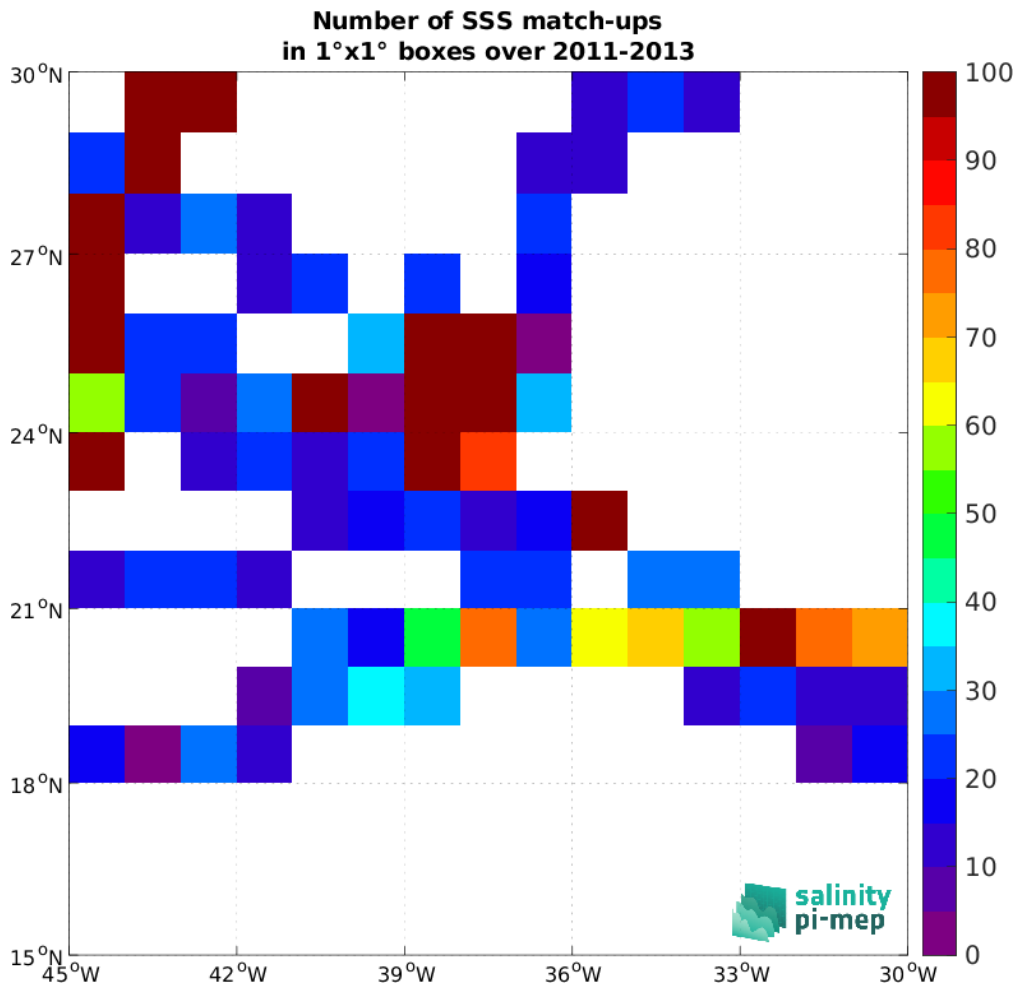
Figure 5: Number of SSS match-ups between TSG (SAMOS) SSS and the Aquarius SSS L4 OI v5 - Weekly (IPRC) SSS product for the SPURS 1 Pi-MEP region over 1^\circ \times 1^\circ boxes and for the full satellite product period.
