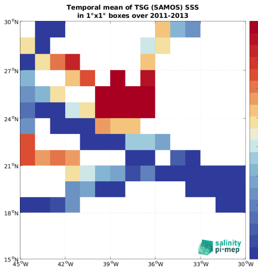
(c) MEAN(TSG (SAMOS) SSS)
