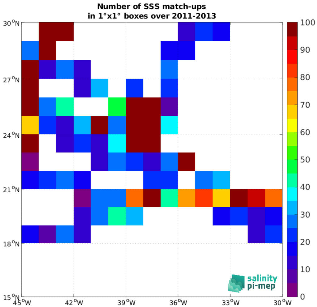
Figure 4: Number of SSS match-ups between TSG (SAMOS) SSS and the Aquarius SSS L4 OI v5 - Weekly (IPRC) SSS product for the SPURS 1 Pi-MEP region over 1^\circ \times 1^\circ boxes and for the full satellite product period.
