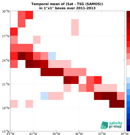
(e) MEAN( \Delta SSS) (Satellite - TSG (SAMOS))
