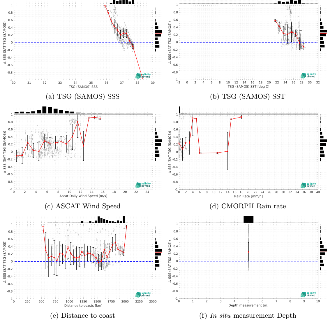
Figure 11: \Delta SSS (Satellite - TSG (SAMOS)) sorted as function of TSG (SAMOS) SSS values a), TSG (SAMOS) SST b), ASCAT Wind speed c), CMORPH rain rate d), distance to coast (e) and in situ measurement depth (f). In all plots the median and Std of \Delta SSS for each bin is indicated by the red curves and black vertical thick bars ( \pm 1 Std)
