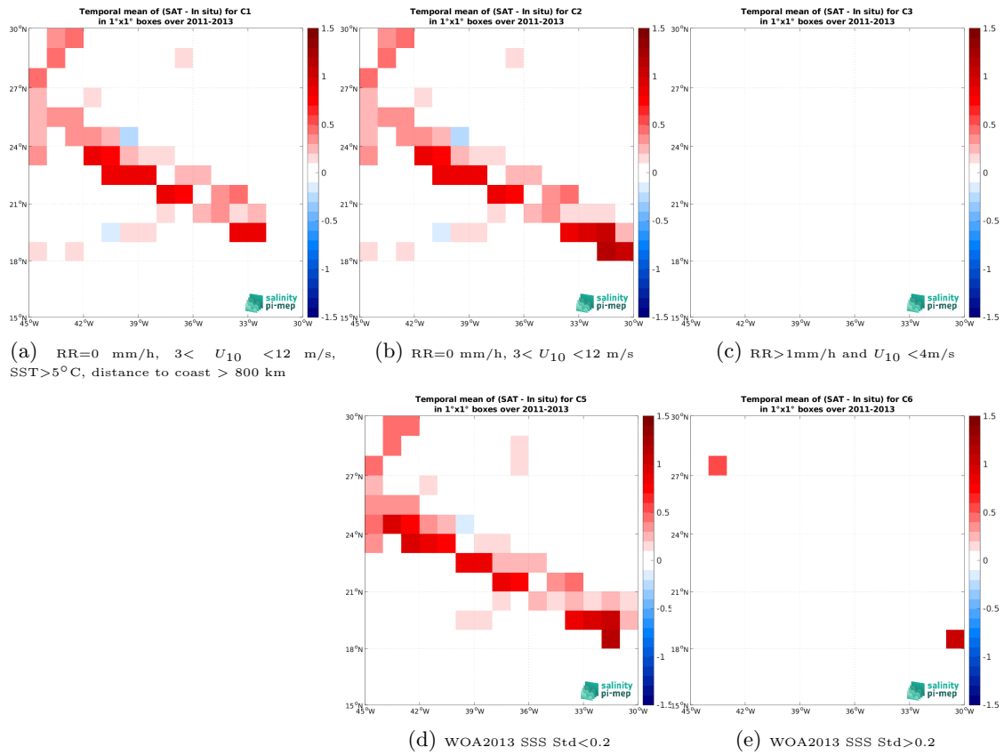
Figure 12: Temporal mean gridded over spatial boxes of size 1^\circ \times 1^\circ of \Delta SSS (Aquarius SSS L4 OI v5 - Weekly (IPRC) - TSG (SAMOS)) for 5 different subdatasets corresponding to:RR=0 mm/h, 3 < U_{10} < 12 m/s, SST >5^\circ C, distance to coast > 800 km (a), RR=0 mm/h, 3 < U_{10} < 12 m/s (b), RR >1 mm/h and U_{10} < 4 m/s (c), WOA2013 SSS Std <0.2 (d), WOA2013 SSS Std >0.2 (e).
