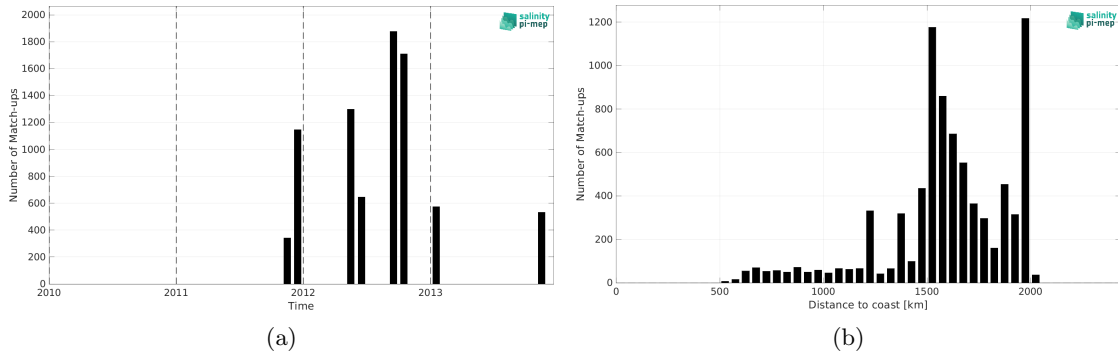
Figure 1: Number of match-ups between TSG (SAMOS) and Aquarius SSS L4 OI v5 - Weekly (IPRC) SSS as a function of time (a) and as function of the distance to coast (b) over the SPURS 1 Pi-MEP region and for the full satellite product period.
