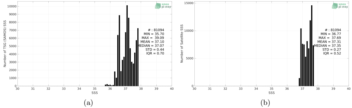
Figure 2: Histograms of SSS from TSG (SAMOS) (a) and Aquarius SSS L4 OI v5 - Weekly (IPRC) (b) considering all match-up pairs per bins of 0.1 over the SPURS 1 Pi-MEP region and for the full satellite product period.
