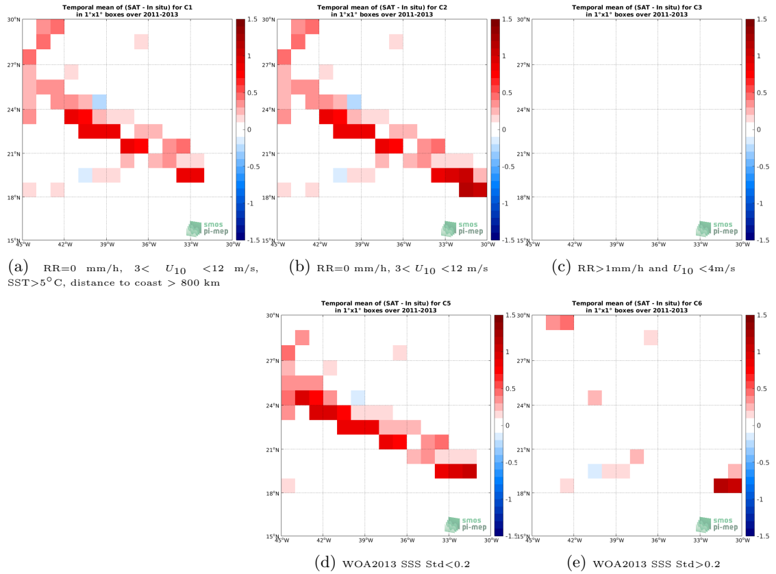
Figure 12: Temporal mean gridded over spatial boxes of size 1^\circ \times 1^\circ of \Delta SSS (Aquarius SSS L4 OI v5 - Weekly (IPRC) - TSG (SAMOS)) for 5 different subdatasets corresponding to: RR=0 mm/h, 3 < U_{10} < 12 m/s, SST > 5^\circ C , distance to coast > 800 km (a), RR=0 mm/h, 3 < U_{10} < 12 m/s (b), RR > 1 mm/h and U_{10} < 4 m/s (c), WOA2013 SSS Std < 0.2 (d), WOA2013 SSS Std > 0.2 (e).
