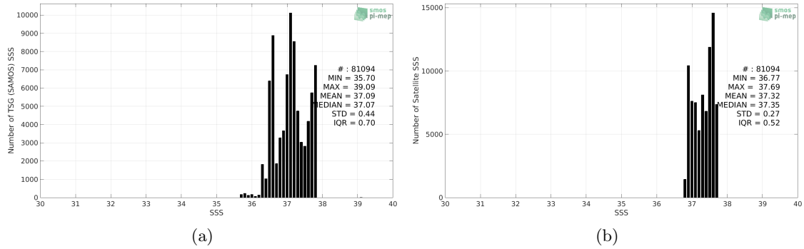
Figure 2: Histograms of SSS from TSG (SAMOS) (a) and Aquarius SSS L4 OI v5 - Weekly (IPRC) (b) considering all match-up pairs per bins of 0.1 over the SPURS 1 Pi-MEP region and for the full satellite product period.
