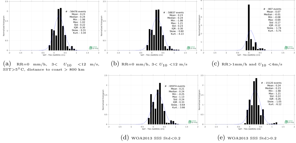
Figure 13: Normalized histogram of \Delta SSS (Aquarius SSS L4 OI v5 - Weekly (IPRC) - TSG (SAMOS)) for 5 different subdatasets corresponding to: RR=0 mm/h, 3 < U_{10} < 12 m/s, SST > 5^\circ C , distance to coast > 800 km (a), RR=0 mm/h, 3 < U_{10} < 12 m/s (b), RR > 1 mm/h and U_{10} < 4 m/s (c), WOA2013 SSS Std < 0.2 (d), WOA2013 SSS Std > 0.2 (e).
