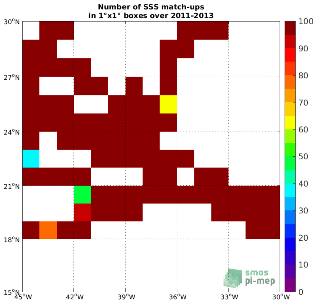
Figure 4: Number of SSS match-ups between TSG (SAMOS) SSS and the Aquarius SSS L4 OI v5 - Weekly (IPRC) SSS product for the SPURS 1 Pi-MEP region over 1°x1° boxes and for the full satellite product period.
