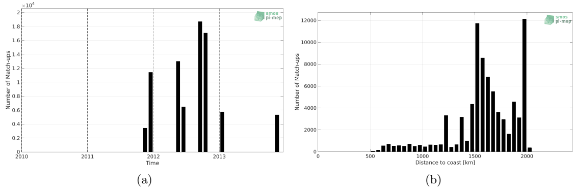
Figure 1: Number of match-ups between TSG (SAMOS) and Aquarius SSS L4 OI v5 - Weekly (IPRC) SSS as a function of time (a) and as function of the distance to coast (b) over the SPURS 1 Pi-MEP region and for the full satellite product period.
