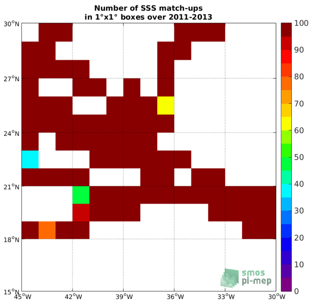
Figure 4: Number of SSS match-ups between TSG-SAMOS SSS and the Aquarius-L4-IPRC-V5-WEEKLY SSS product for the SPURS 1 Pi-MEP region over 1°x1° boxes and for the full satellite product period.
