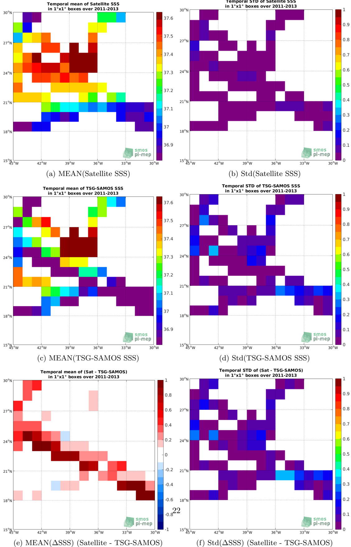
Figure 6: Temporal mean (left) and Std (right) of SSS from Aquarius-L4-IPRC-V5-WEEKLY (top), TSG-SAMOS (middle), and of \Delta SSS (Satellite - TSG-SAMOS). Only match-up pairs are used to generate these maps.
