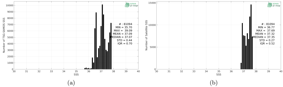
Figure 2: Histograms of SSS from TSG-SAMOS (a) and Aquarius-L4-IPRC-V5-WEEKLY (b) considering all match-up pairs per bins of 0.1 over the SPURS 1 Pi-MEP region and for the full satellite product period.
