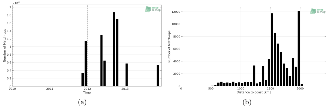
Figure 1: Number of match-ups between TSG-SAMOS and Aquarius-L4-IPRC-V5-WEEKLY SSS as a function of time (a) and as function of the distance to coast (b) over the SPURS 1 Pi-MEP region and for the full satellite product period.
