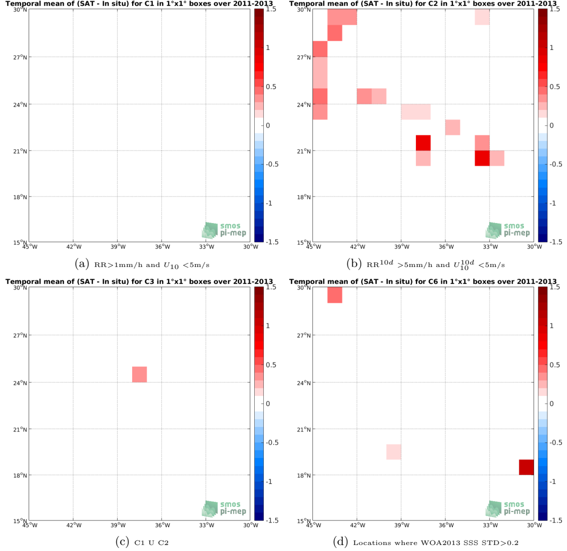
Figure 12: Temporal mean gridded over spatial boxes of size 1^\circ \times 1^\circ of \Delta SSS (Aquarius-L4-IPRC-V5-WEEKLY - TSG-SAMOS) for 4 different subdatasets corresponding to: RR > 1\text{mm/h} and U_{10} < 5\text{m/s} (a), RR^{10d} > 5\text{mm/h} and U_{10}^{10d} < 5\text{m/s} (b), C1 U C2 (c), Locations where WOA2013 SSS STD > 0.2 (d).
