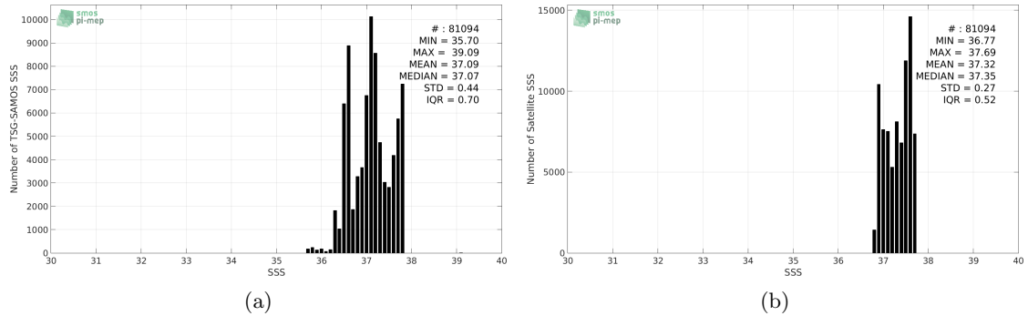
Figure 2: Histograms of SSS from TSG-SAMOS (a) and Aquarius-L4-IPRC-V5-WEEKLY (b) considering all match-up pairs per bins of 0.1 over the SPURS 1 Pi-MEP region and for the full satellite product period.
