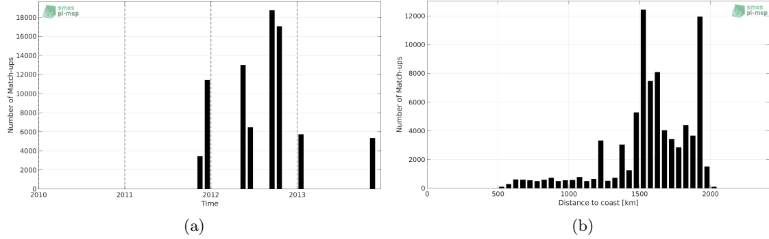
Figure 1: Number of match-ups between TSG-SAMOS and Aquarius-L4-IPRC-V5-WEEKLY SSS as a function of time (a) and as function of the distance to coast (b) over the SPURS 1 Pi-MEP region and for the full satellite product period.
