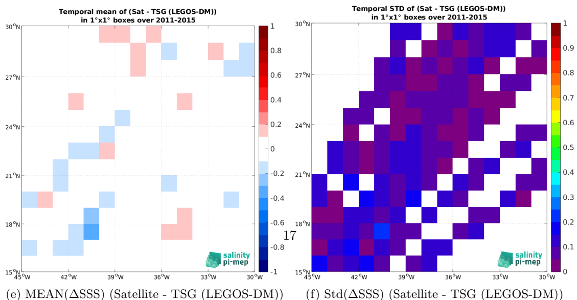
Figure 7: Temporal mean (left) and Std (right) of SSS from Aquarius SSS L4 OI v5 - Weekly (IPRC) (top), TSG (LEGOS-DM) (middle), and of \Delta SSS (Satellite - TSG (LEGOS-DM)). Only match-up pairs are used to generate these maps.
