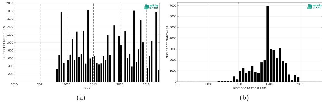
Figure 2: Number of match-ups between TSG (LEGOS-DM) and Aquarius SSS L4 OI v5 - Weekly (IPRC) SSS as a function of time (a) and as function of the distance to coast (b) over the SPURS 1 Pi-MEP region and for the full satellite product period.
