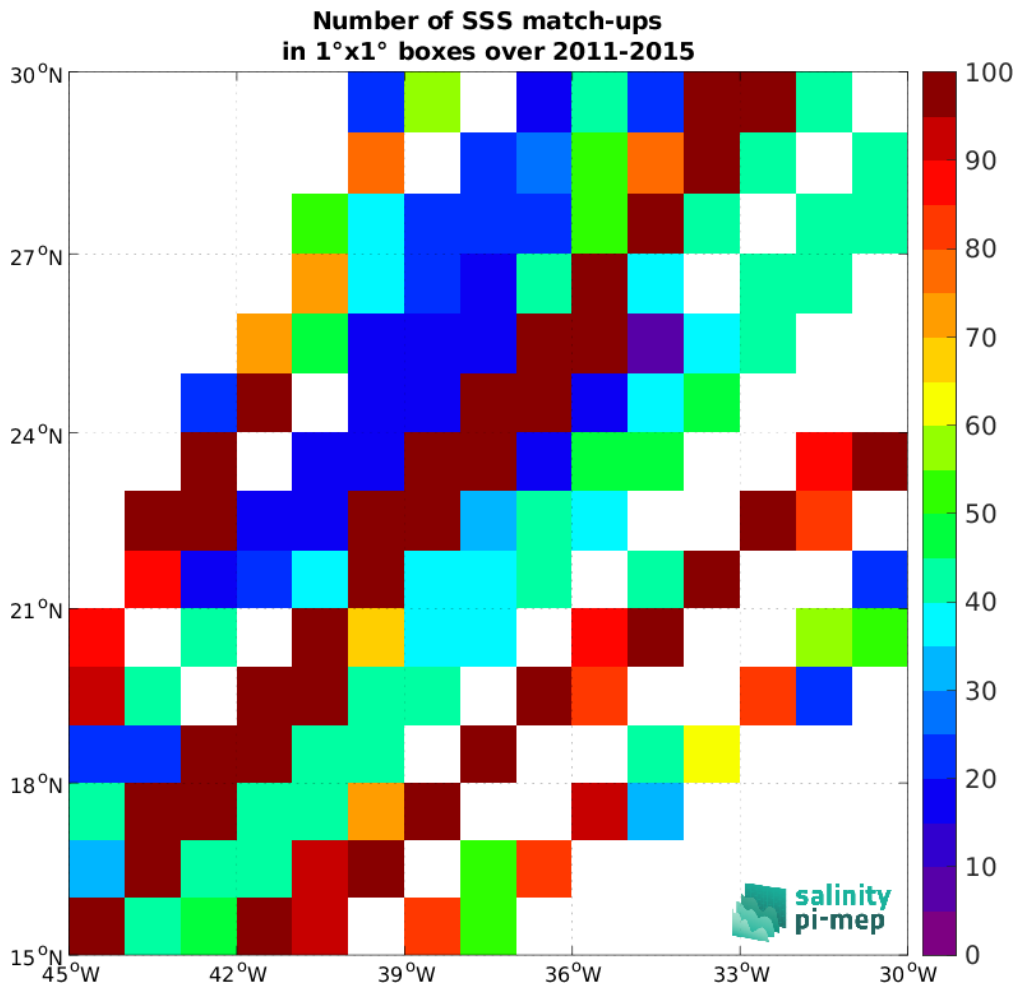
Figure 5: Number of SSS match-ups between TSG (LEGOS-DM) SSS and the Aquarius SSS L4 OI v5 - Weekly (IPRC) SSS product for the SPURS 1 Pi-MEP region over 1^\circ \times 1^\circ boxes and for the full satellite product period.
