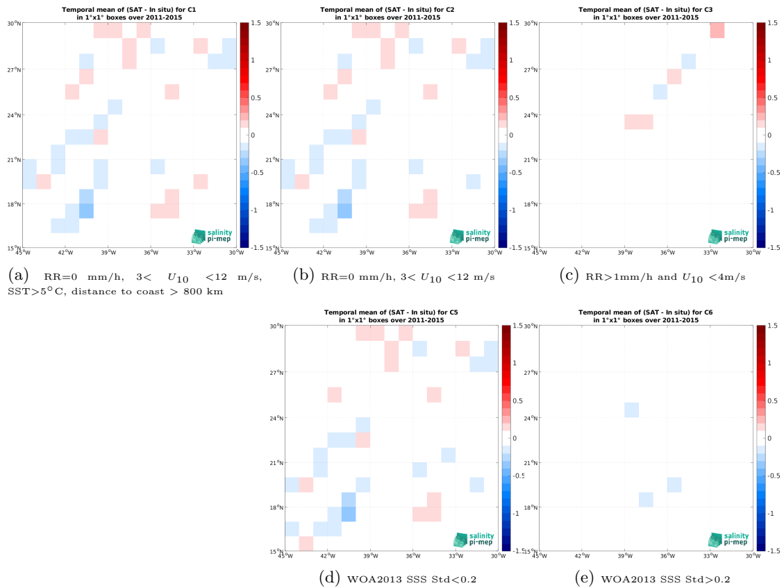
Figure 14: Temporal mean gridded over spatial boxes of size 1^\circ \times 1^\circ of \Delta\text{SSS} (Aquarius SSS L4 OI v5 - Weekly (IPRC) - TSG (LEGOS-DM)) for 5 different subdatasets corresponding to:RR=0 mm/h, 3 < U_{10} < 12 m/s, SST>5°C, distance to coast > 800 km (a), RR=0 mm/h, 3 < U_{10} < 12 m/s (b), RR>1mm/h and U_{10} < 4 m/s (c), WOA2013 SSS Std<0.2 (d), WOA2013 SSS Std>0.2 (e).
