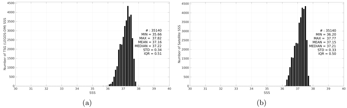
Figure 3: Histograms of SSS from TSG (LEGOS-DM) (a) and Aquarius SSS L4 OI v5 - Weekly (IPRC) (b) considering all match-up pairs per bins of 0.1 over the SPURS 1 Pi-MEP region and for the full satellite product period.
