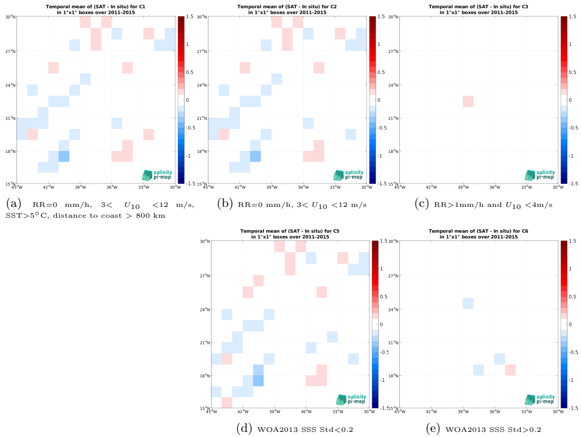
Figure 12: Temporal mean gridded over spatial boxes of size 1^\circ \times 1^\circ of \Delta\text{SSS} (Aquarius SSS L4 OI v5 - Weekly (IPRC) - TSG (LEGOS-DM)) for 5 different subdatasets corresponding to:RR=0 mm/h, 3 < U_{10} < 12 m/s, SST > 5^\circ\text{C} , distance to coast > 800 km (a), RR=0 mm/h, 3 < U_{10} < 12 m/s (b), RR > 1\text{mm/h} and U_{10} < 4\text{m/s} (c), WOA2013 SSS Std < 0.2 (d), WOA2013 SSS Std > 0.2 (e).
