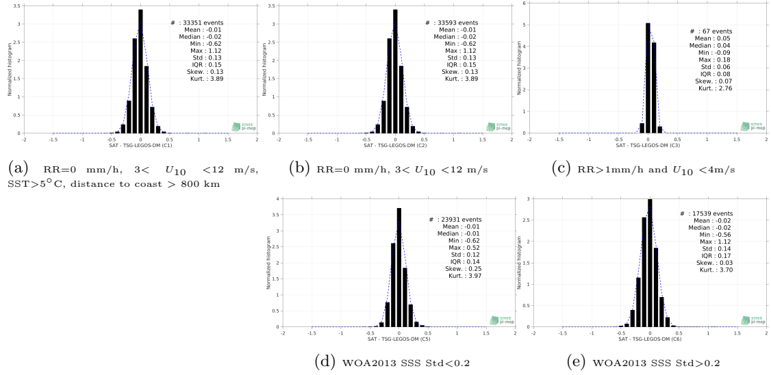
Figure 13: Normalized histogram of \Delta SSS (Aquarius-L4-IPRC-V5-WEEKLY - TSG-LEGOS-DM) for 5 different subdatasets corresponding to: RR=0 mm/h, 3 < U_{10} < 12 m/s, SST>5°C, distance to coast > 800 km (a), RR=0 mm/h, 3 < U_{10} < 12 m/s (b), RR>1mm/h and U_{10} < 4 m/s (c), WOA2013 SSS Std<0.2 (d), WOA2013 SSS Std>0.2 (e).
