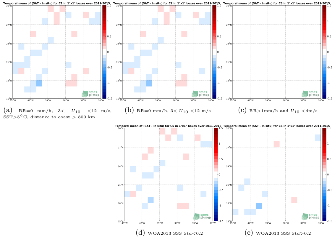
Figure 12: Temporal mean gridded over spatial boxes of size 1^\circ \times 1^\circ of \Delta SSS (Aquarius-L4-IPRC-V5-WEEKLY - TSG-LEGOS-DM) for 5 different subdatasets corresponding to:RR=0 mm/h, 3 < U_{10} < 12 m/s, SST > 5^\circ C , distance to coast > 800 km (a), RR=0 mm/h, 3 < U_{10} < 12 m/s (b), RR > 1 mm/h and U_{10} < 4 m/s (c), WOA2013 SSS Std < 0.2 (d), WOA2013 SSS Std > 0.2 (e).
