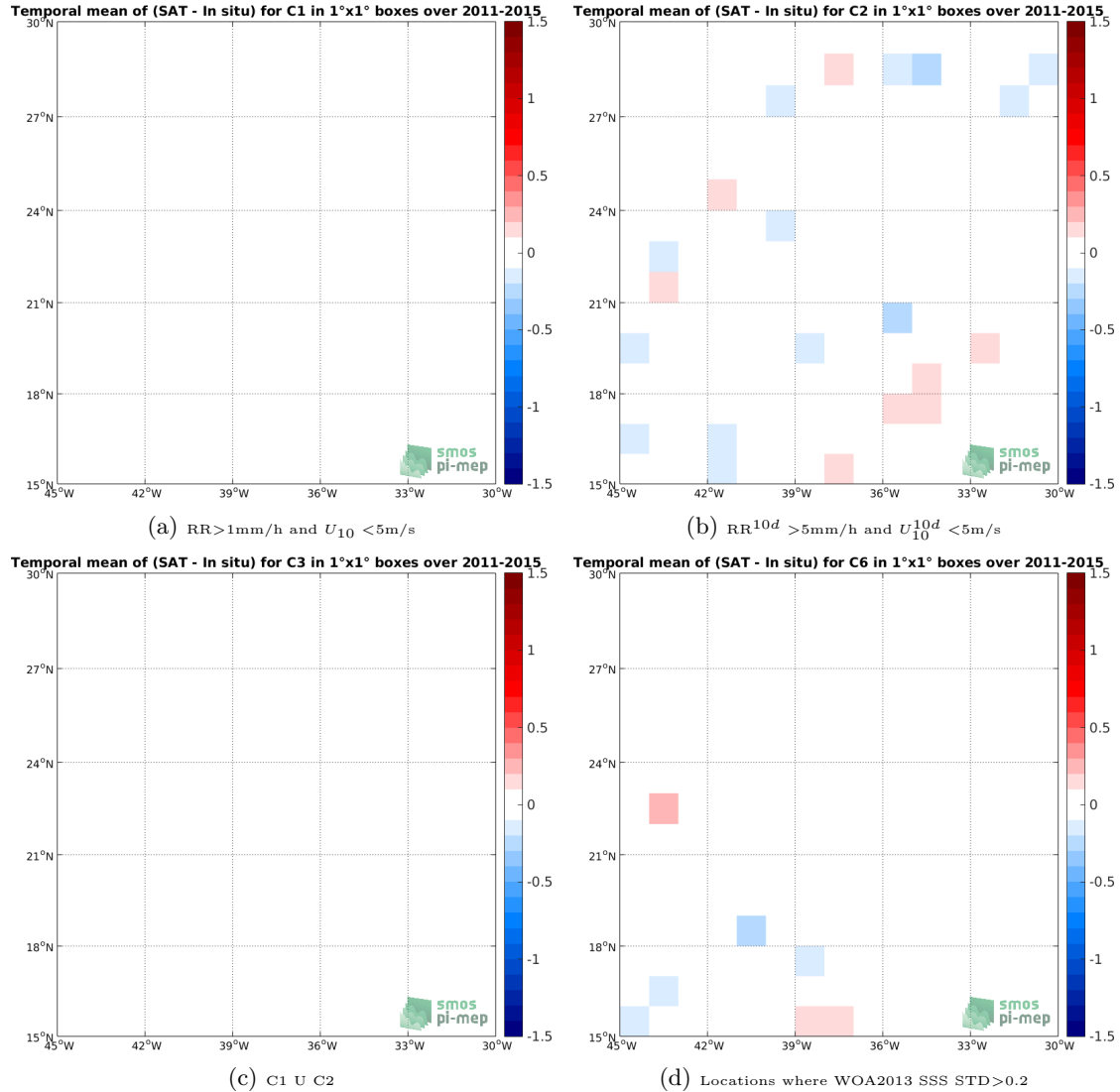
Figure 12: Temporal mean gridded over spatial boxes of size 1^\circ \times 1^\circ of \Delta SSS (Aquarius-L4-IPRC-V5-WEEKLY - TSG-LEGOS-DM) for 4 different subdatasets corresponding to: RR > 1mm/h and U_{10} < 5\text{m/s} (a), RR 10d > 5mm/h and U_{10}^{10d} < 5\text{m/s} (b), C1 U C2 (c), Locations where WOA2013 SSS STD > 0.2 (d).
