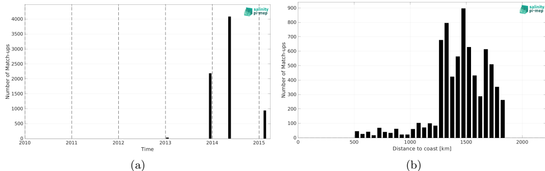
Figure 2: Number of match-ups between TSG (GOSUD-Sailing-ship) and Aquarius SSS L4 OI v5 - Weekly (IPRC) SSS as a function of time (a) and as function of the distance to coast (b) over the SPURS 1 Pi-MEP region and for the full satellite product period.
