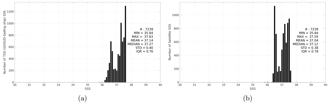
Figure 3: Histograms of SSS from TSG (GOSUD-Sailing-ship) (a) and Aquarius SSS L4 OI v5 - Weekly (IPRC) (b) considering all match-up pairs per bins of 0.1 over the SPURS 1 Pi-MEP region and for the full satellite product period.
