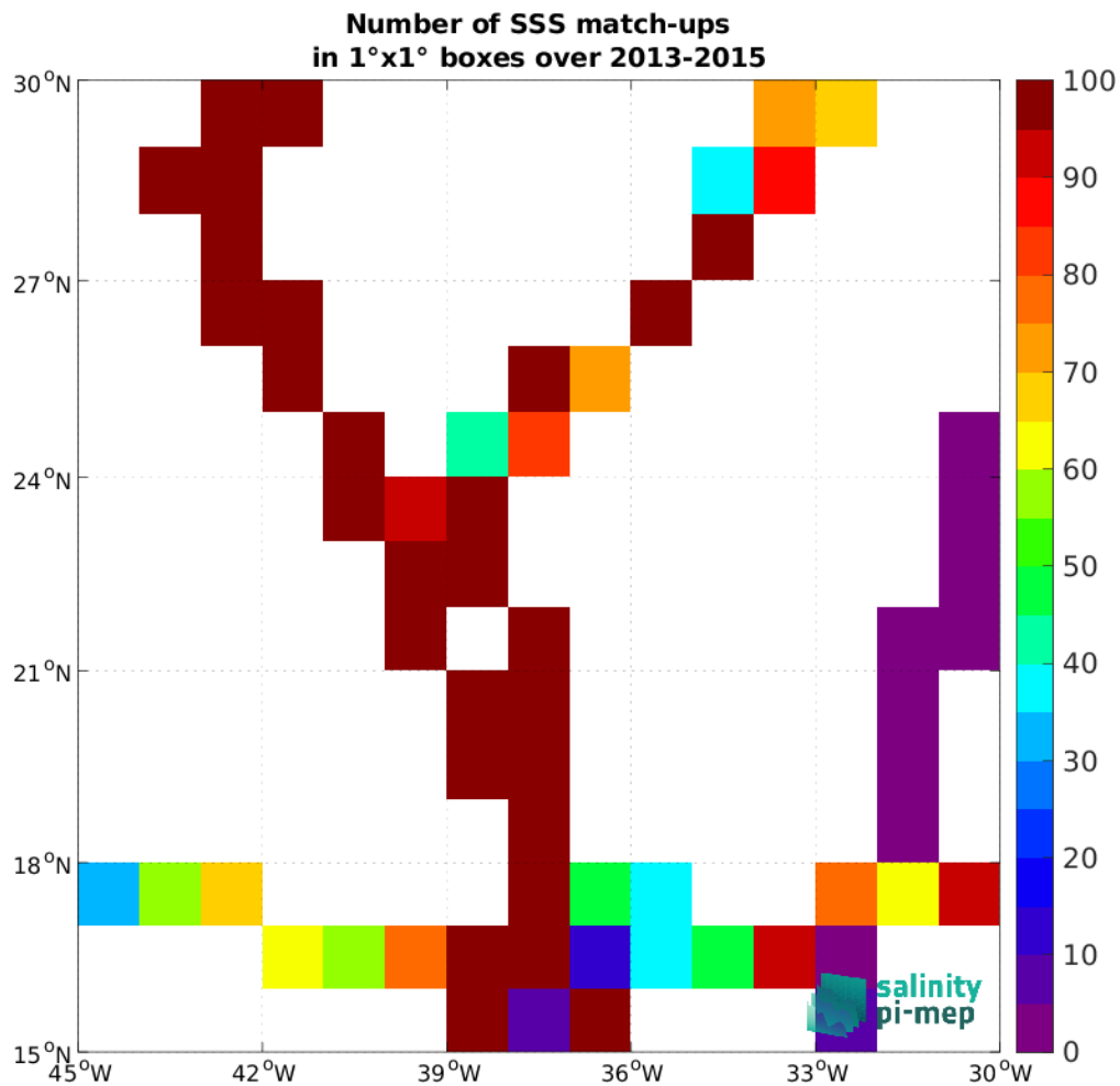
Figure 5: Number of SSS match-ups between TSG (GOSUD-Sailing-ship) SSS and the Aquarius SSS L4 OI v5 - Weekly (IPRC) SSS product for the SPURS 1 Pi-MEP region over 1^\circ \times 1^\circ boxes and for the full satellite product period.
