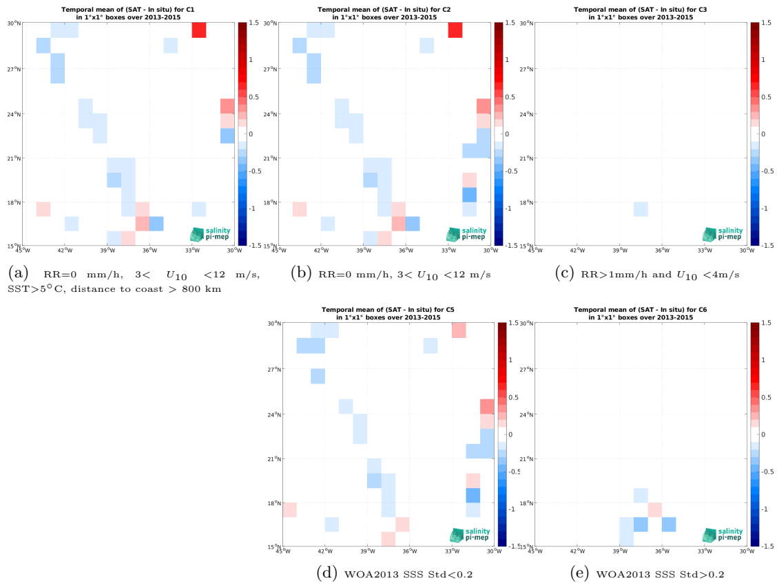
Figure 14: Temporal mean gridded over spatial boxes of size 1^\circ \times 1^\circ of \Delta\text{SSS} (Aquarius SSS L4 OI v5 - Weekly (IPRC) - TSG (GOSUD-Sailing-ship)) for 5 different subdatasets corresponding to:RR=0 mm/h, 3 < U_{10} < 12 m/s, SST>5°C, distance to coast > 800 km (a), RR=0 mm/h, 3 < U_{10} < 12 m/s (b), RR>1mm/h and U_{10} < 4 m/s (c), WOA2013 SSS Std<0.2 (d), WOA2013 SSS Std>0.2 (e).
