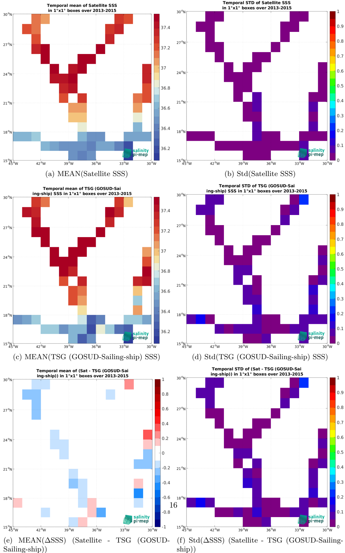
Figure 7: Temporal mean (left) and Std (right) of SSS from Aquarius SSS L4 OI v5 - Weekly (IPRC) (top), TSG (GOSUD-Sailing-ship) (middle), and of \Delta SSS (Satellite - TSG (GOSUD-Sailing-ship)). Only match-up pairs are used to generate these maps.
