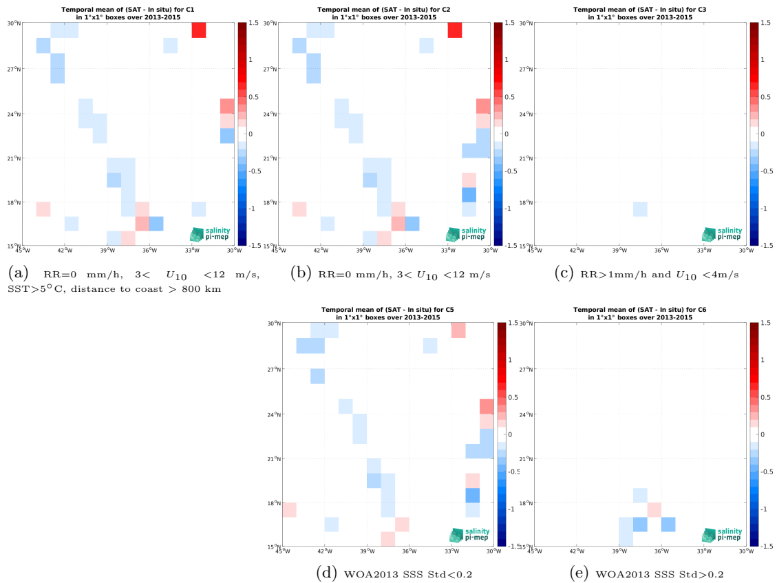
Figure 14: Temporal mean gridded over spatial boxes of size 1^\circ \times 1^\circ of \Delta SSS (Aquarius SSS L4 OI v5 - Weekly (IPRC) - TSG (GOSUD-Sailing-ship)) for 5 different subdatasets corresponding to:RR=0 mm/h, 3 < U_{10} < 12 m/s, SST >5^\circ C, distance to coast > 800 km (a), RR=0 mm/h, 3 < U_{10} < 12 m/s (b), RR >1 mm/h and U_{10} < 4 m/s (c), WOA2013 SSS Std <0.2 (d), WOA2013 SSS Std >0.2 (e).
