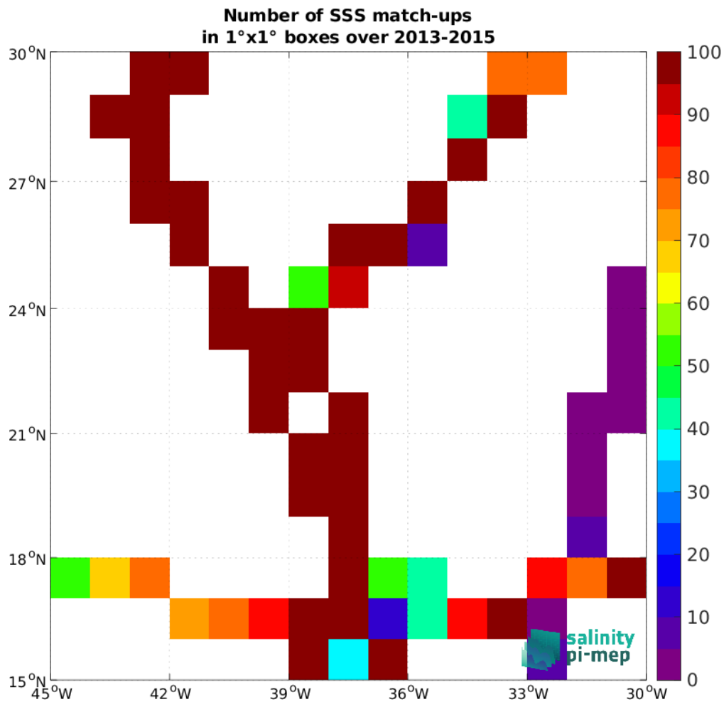
Figure 4: Number of SSS match-ups between TSG (GOSUD-Sailing-ship) SSS and the Aquarius SSS L4 OI v5 - Weekly (IPRC) SSS product for the SPURS 1 Pi-MEP region over 1^\circ \times 1^\circ boxes and for the full satellite product period.
