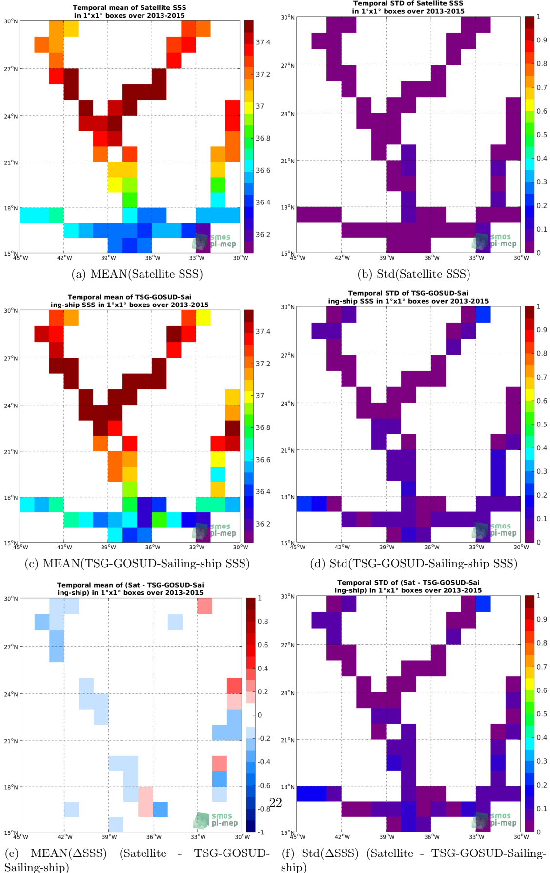
Figure 6: Temporal mean (left) and Std (right) of SSS from Aquarius-L4-IPRC-V5-WEEKLY (top), TSG-GOSUD-Sailing-ship (middle), and of \Delta SSS (Satellite - TSG-GOSUD-Sailing-ship). Only match-up pairs are used to generate these maps.
