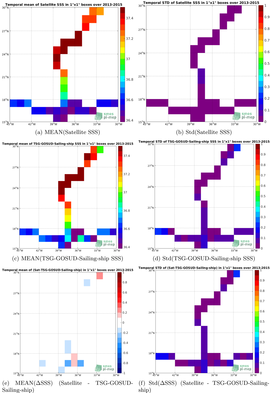
Figure 6: Temporal mean (left) and Std (right) of SSS from Aquarius-L4-IPRC-V5-WEEKLY (top), TSG-GOSUD-Sailing-ship (middle), and of \Delta SSS (Satellite - TSG-GOSUD-Sailing-ship). Only match-up pairs are used to generate these maps.
