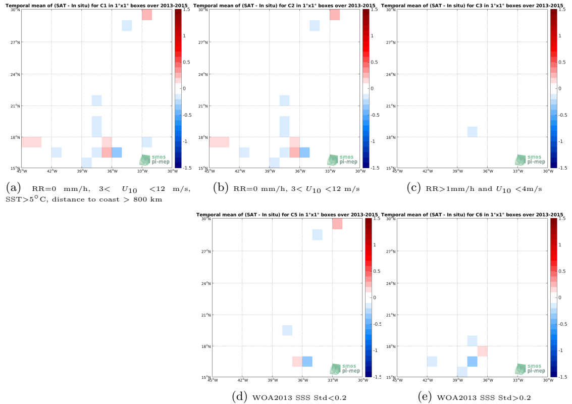
Figure 12: Temporal mean gridded over spatial boxes of size 1^\circ \times 1^\circ of \Delta SSS (Aquarius-L4-IPRC-V5-WEEKLY - TSG-GOSUD-Sailing-ship) for 5 different subdatasets corresponding to: RR=0 mm/h, 3 < U_{10} < 12 m/s, SST > 5^\circ\text{C} , distance to coast > 800 km (a), RR=0 mm/h, 3 < U_{10} < 12 m/s (b), RR > 1 mm/h and U_{10} < 4 m/s (c), WOA2013 SSS Std < 0.2 (d), WOA2013 SSS Std > 0.2 (e).
